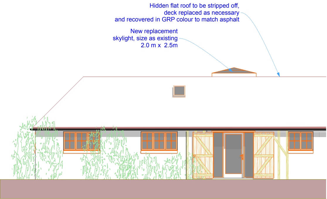
North Elevation
