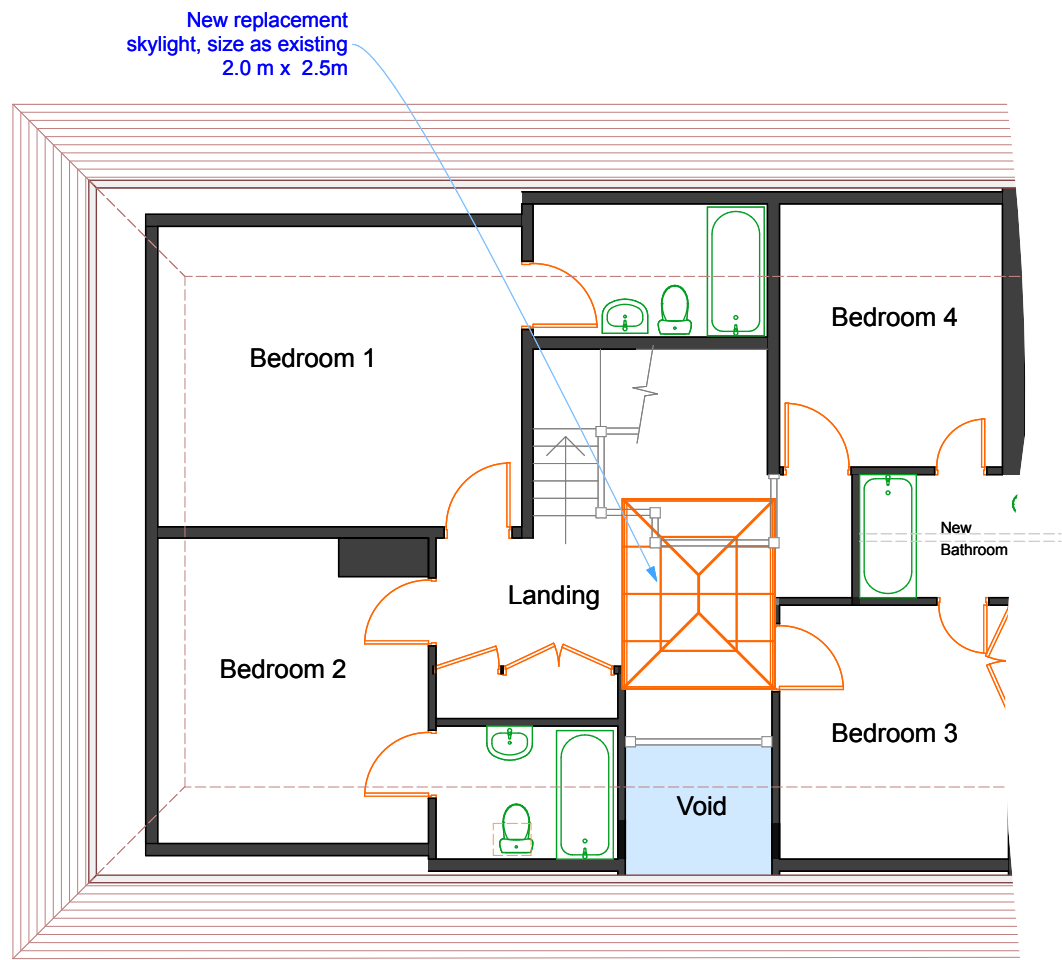
First Floor
