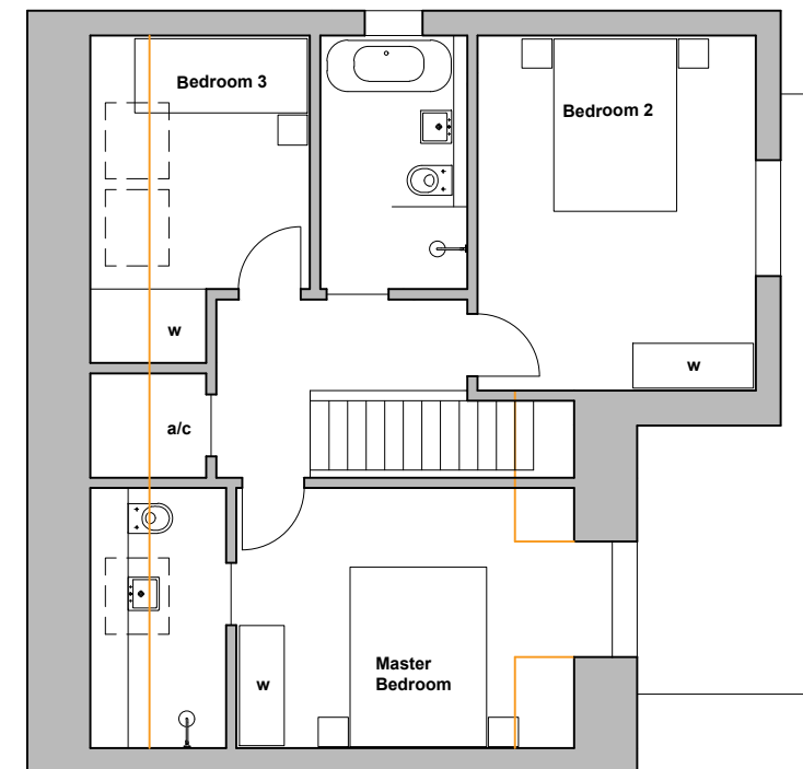
PLOT 2 FLOOR PLANS SCALE 1:100 @ a3
