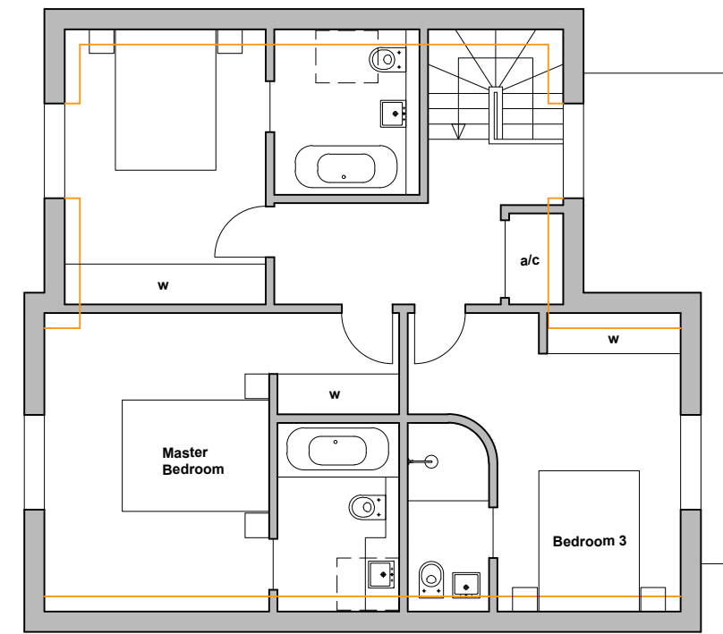
PLOT 1 FLOOR PLANS SCALE 1:100 @ a3
