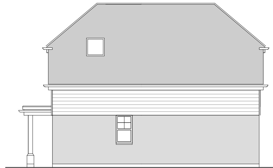
SIDE ELEVATION (NORTH)
