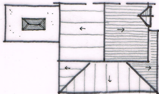
ROOF PLAN 1:200
