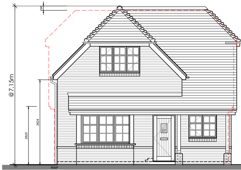
Front Elevation
