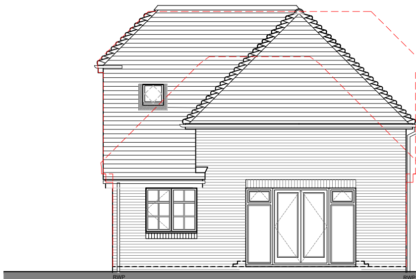
Rear elevation
