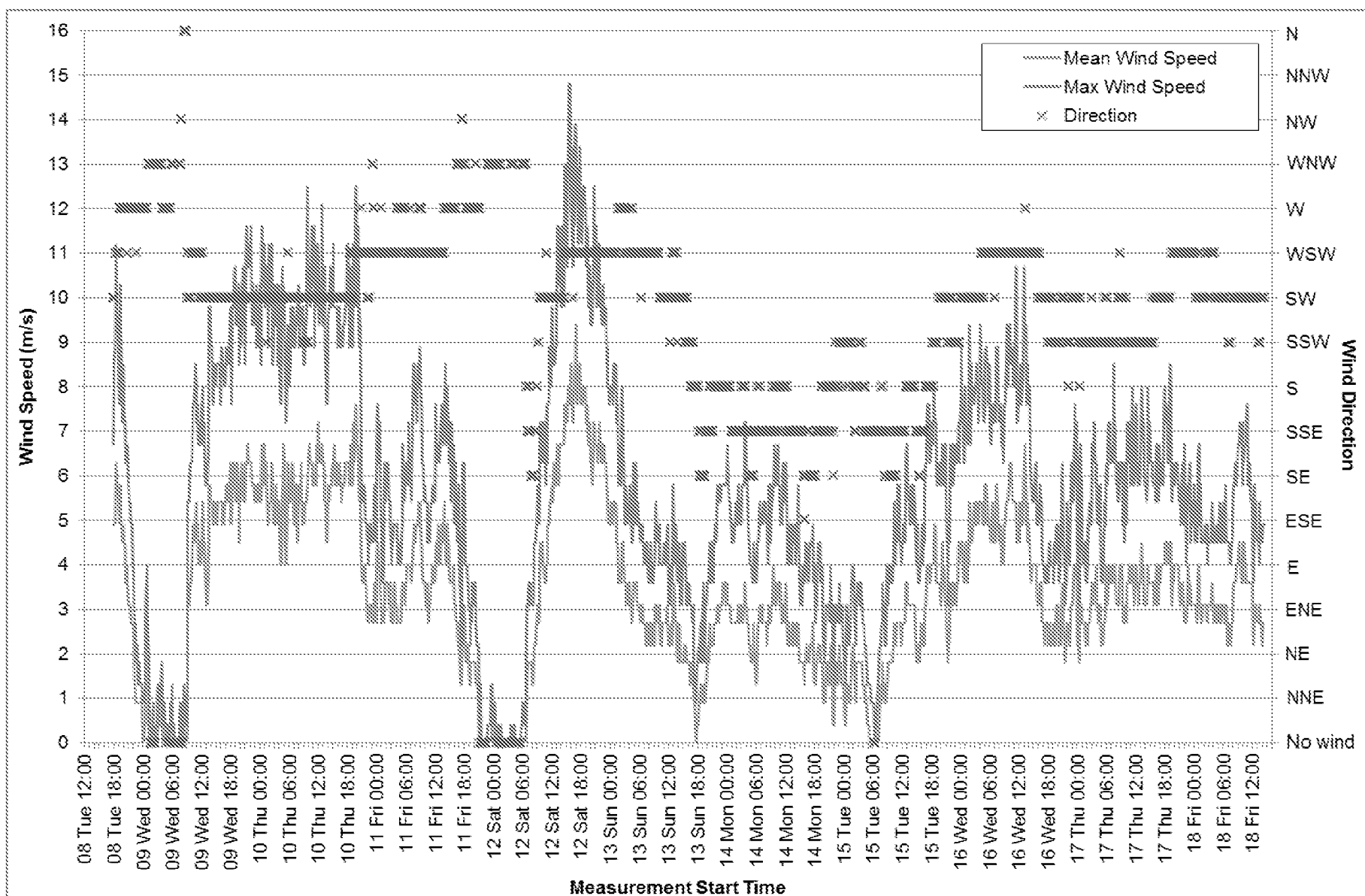
FIGURE A6: UNATTENDED CONTINUOUS WEATHER MONITORING RESULTS AT LT1, TUESDAY 8 TH DECEMBER TO FRIDAY 18 TH DECEMBER 2015
