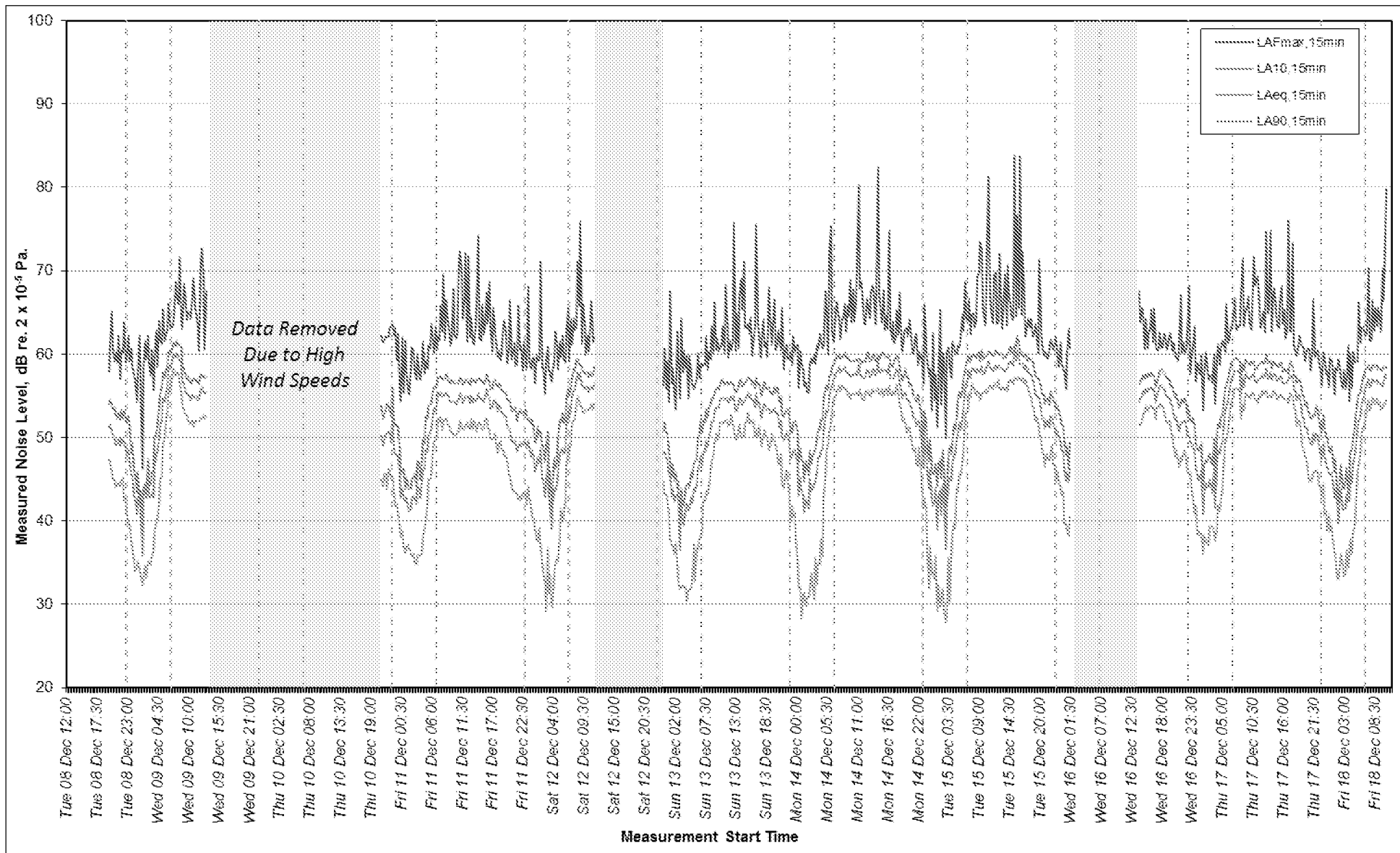
FIGURE A3: UNATTENDED CONTINUOUS NOISE MONITORING RESULTS AT LT1, TUESDAY 8 TH DECEMBER TO FRIDAY 18 TH DECEMBER 2015
