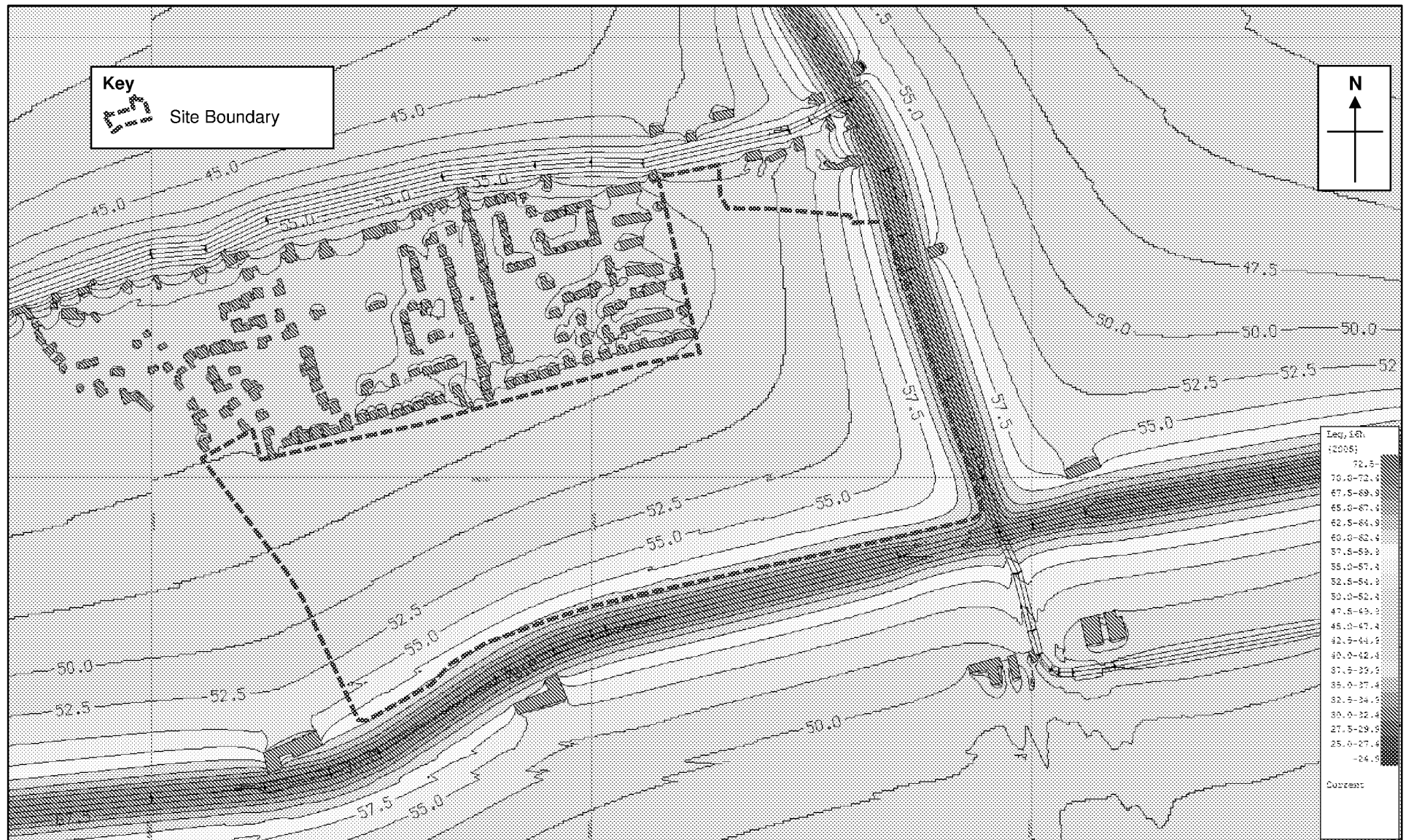
FIGURE A9: LAEQ,16HR CONTOUR PLOT (FREE-FIELD) WITH CURRENT TRAFFIC CONDITIONS
