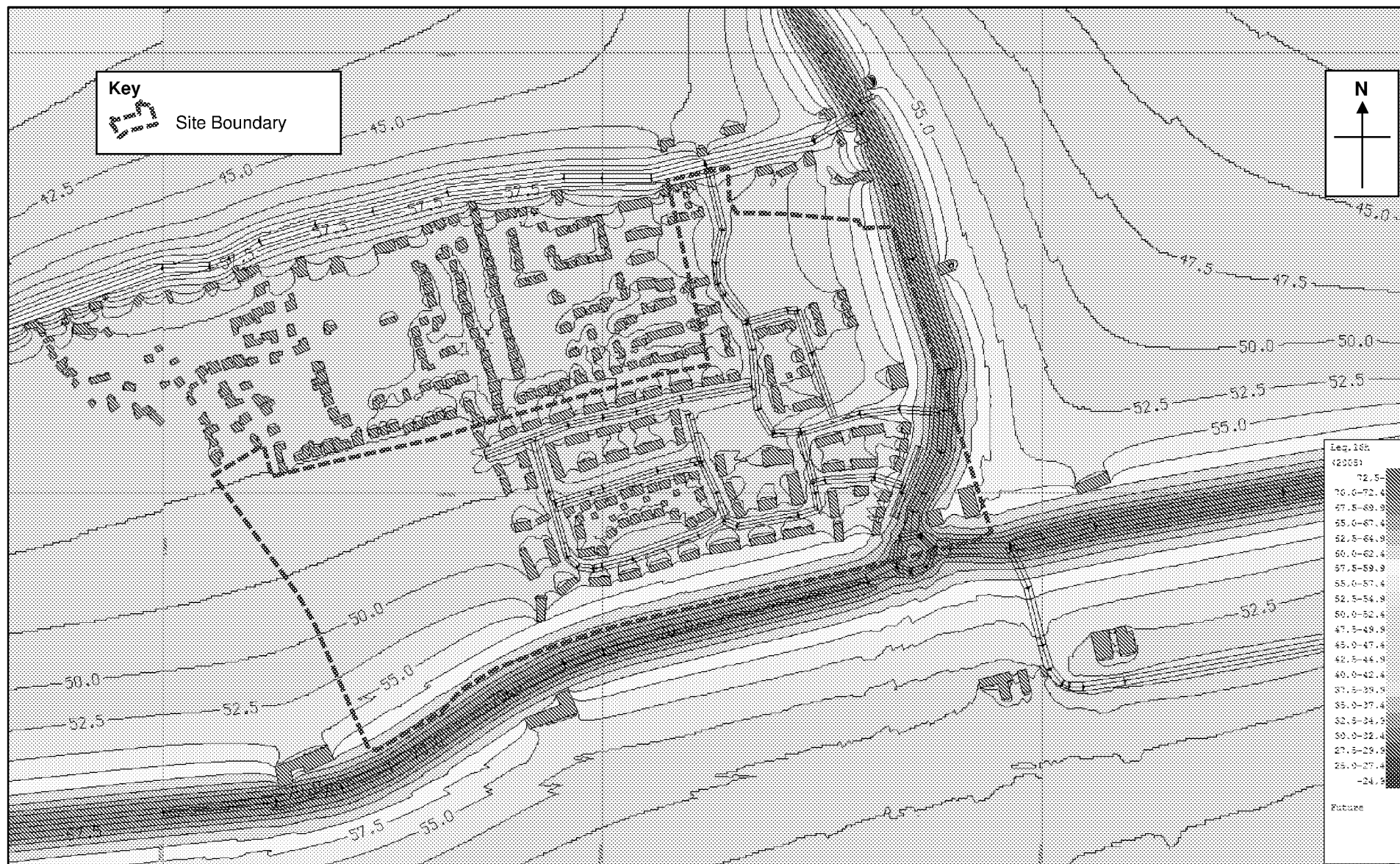
FIGURE A10: LAEQ,16HR CONTOUR PLOT (FREE-FIELD) WITH FUTURE TRAFFIC CONDITIONS
