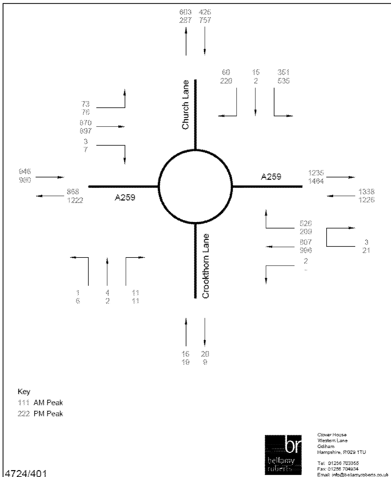
FIGURE A7: EXISTING AM/PM PEAK HOUR TRAFFIC FLOWS
