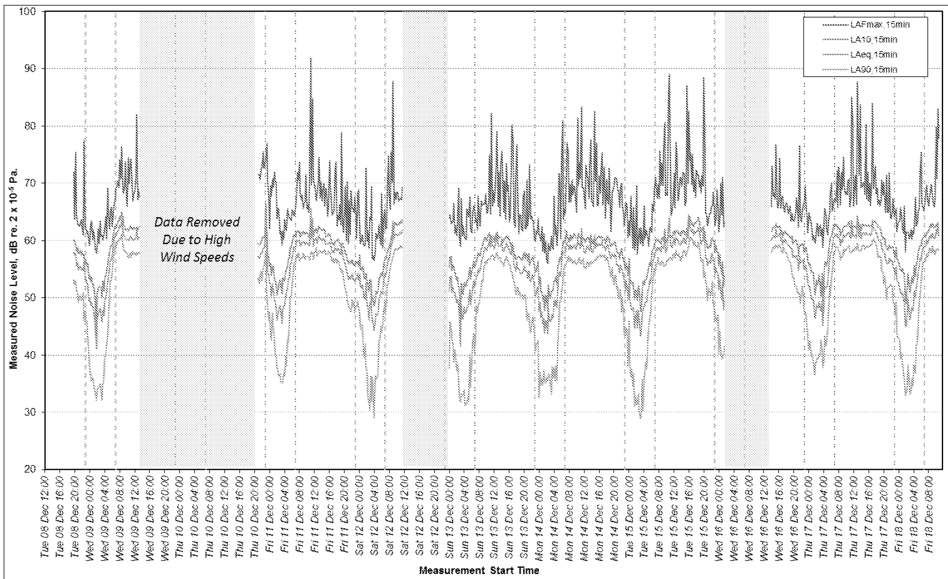
FIGURE A5: UNATTENDED CONTINUOUS NOISE MONITORING RESULTS AT LT3, TUESDAY 8 TH DECEMBER TO FRIDAY 18 TH DECEMBER 2015
