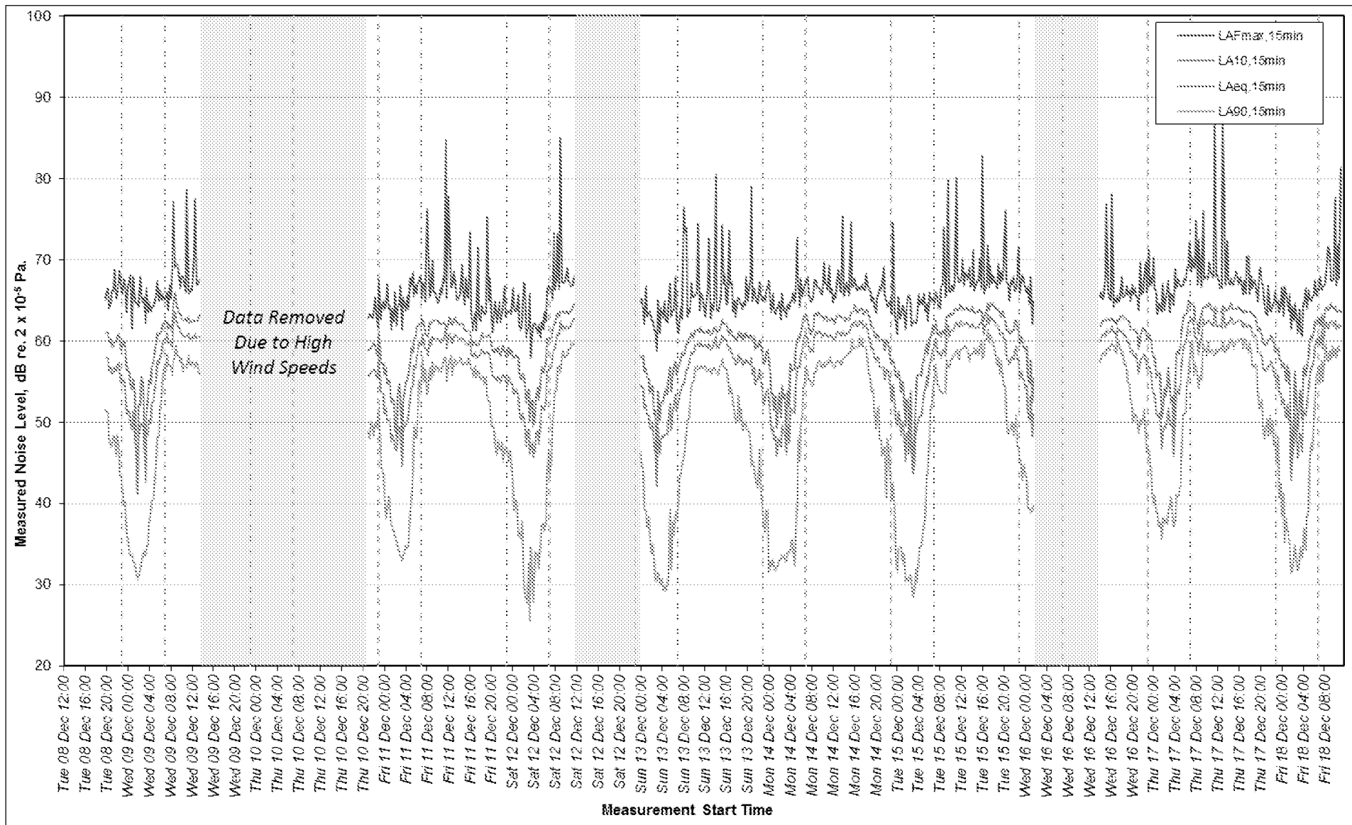
FIGURE A4: UNATTENDED CONTINUOUS NOISE MONITORING RESULTS AT LT2, TUESDAY 8 TH DECEMBER TO FRIDAY 18 TH DECEMBER 2015
