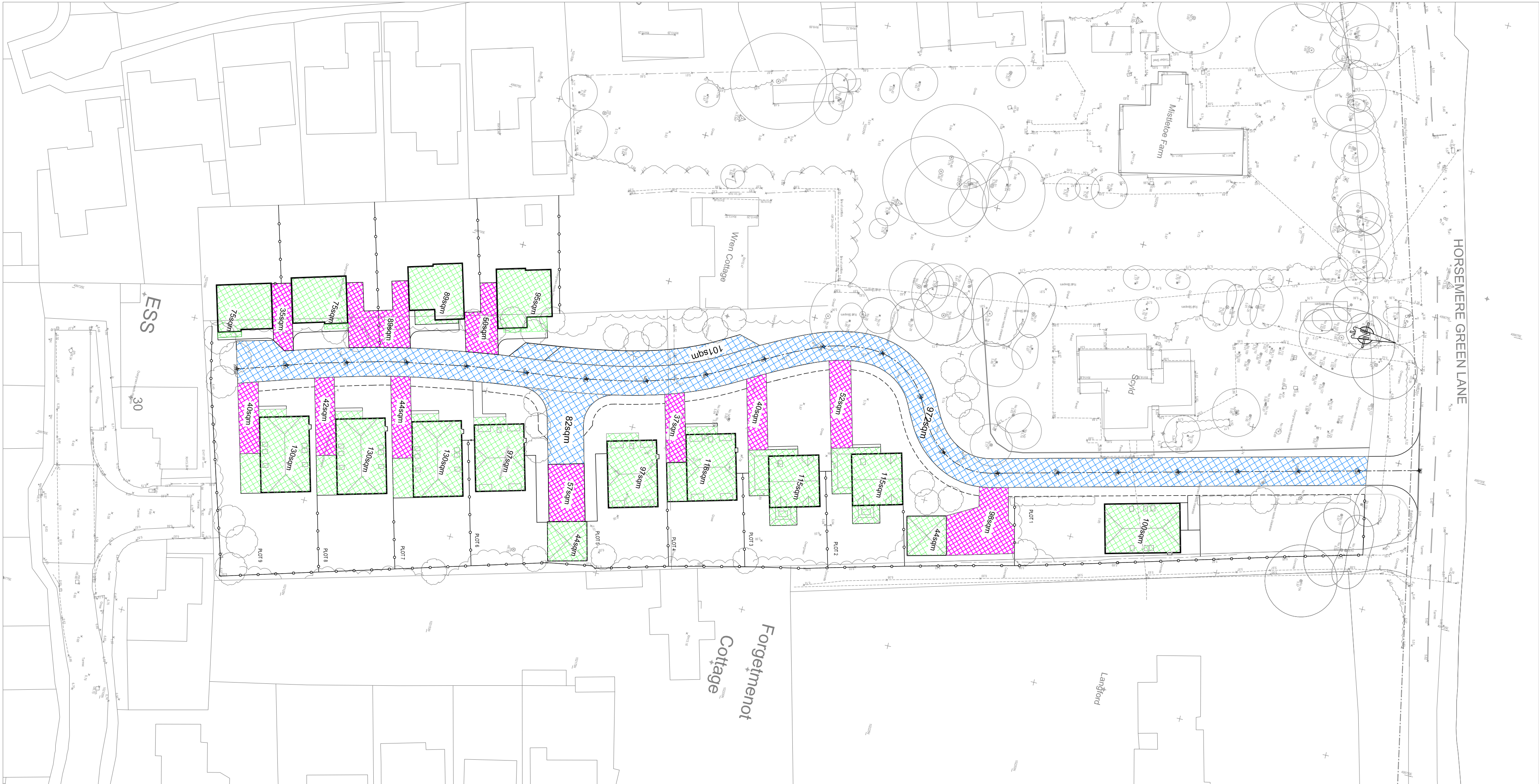
Proposed Impermeable Areas - Scale 1:500
