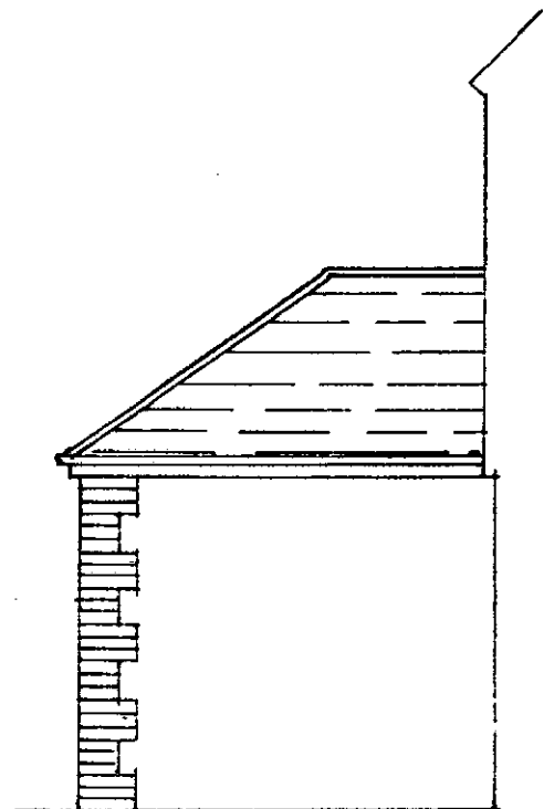
SIDE (WEST) ELEVATION Scale 1:50
