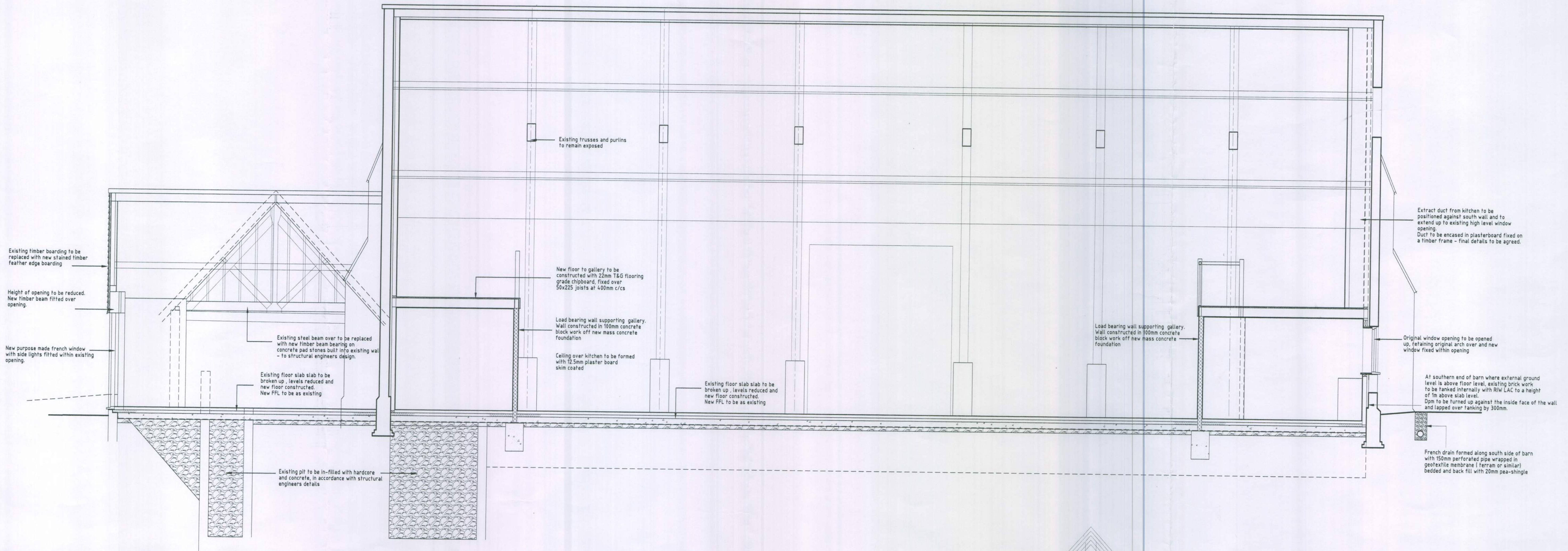
Section EE
