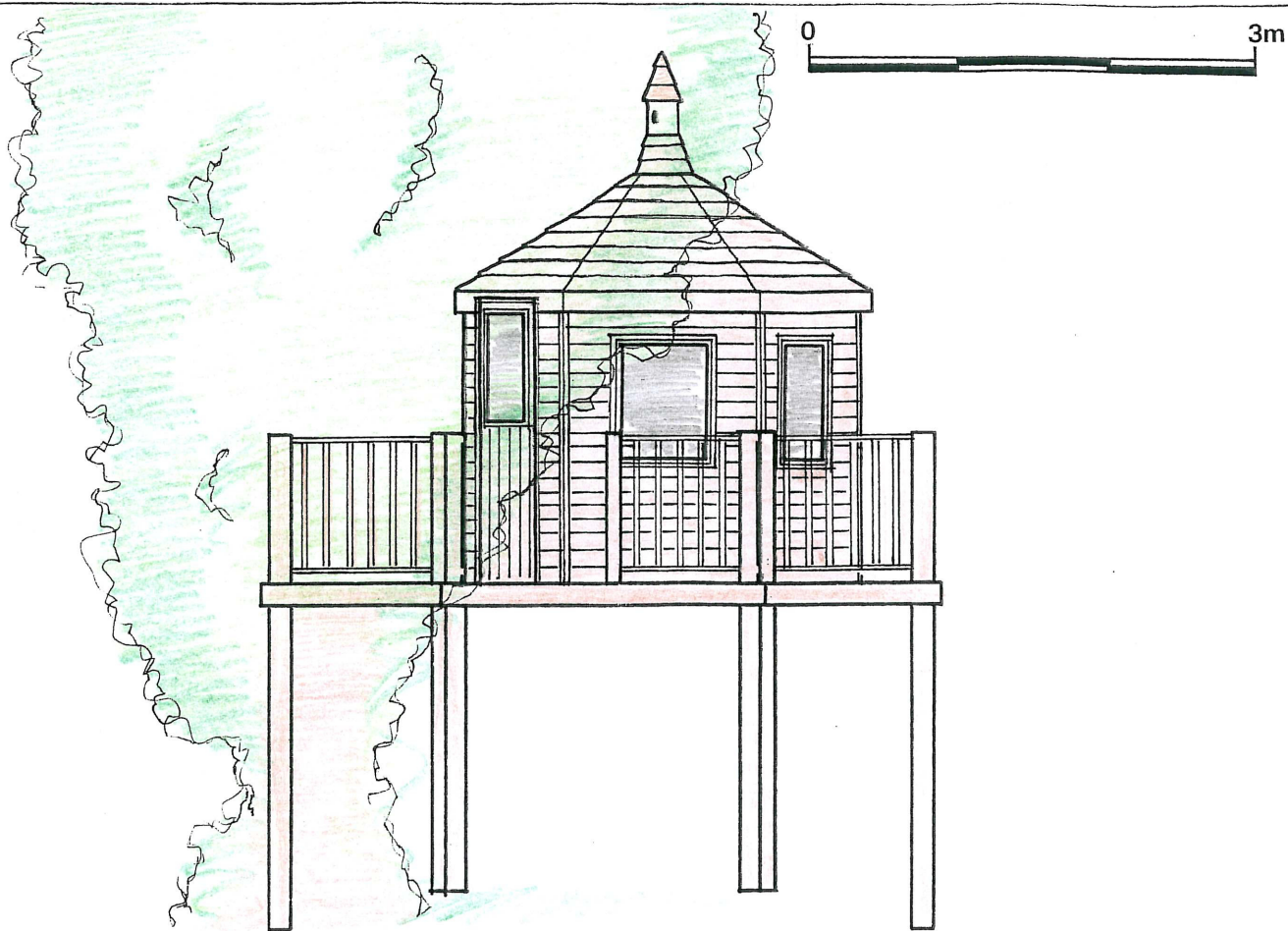
EAST ELEVATION AS EXISTING
