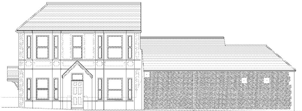
Fig 5. Proposed front (east) elevation
