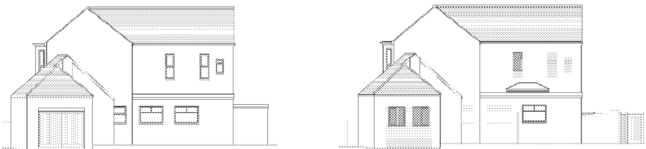
Fig 6. Existing and proposed side (north) elevation
