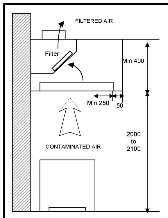
Figure 4.4 Canopy dimensions
