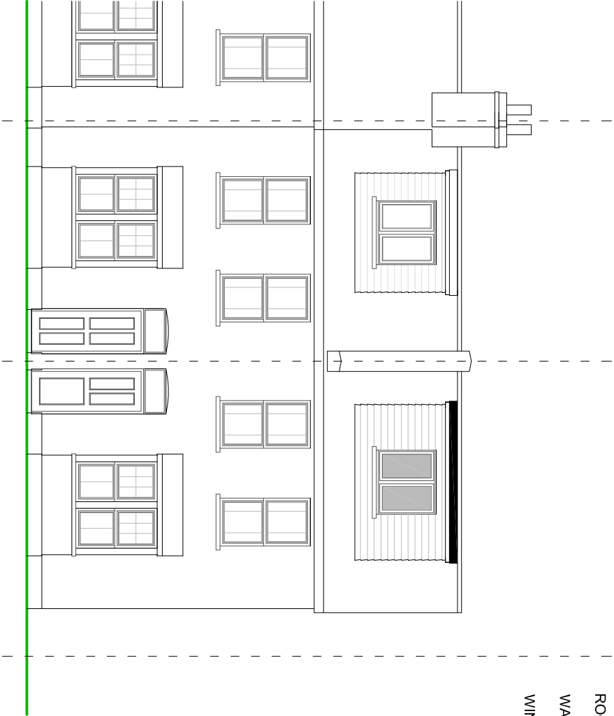
SIDE ELEVATION
