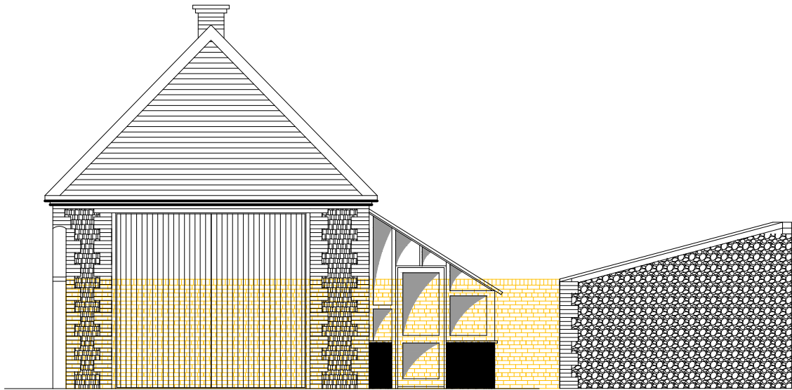
PROPOSED SOUTH ELEVATION - showing garden walls (new & extg)
