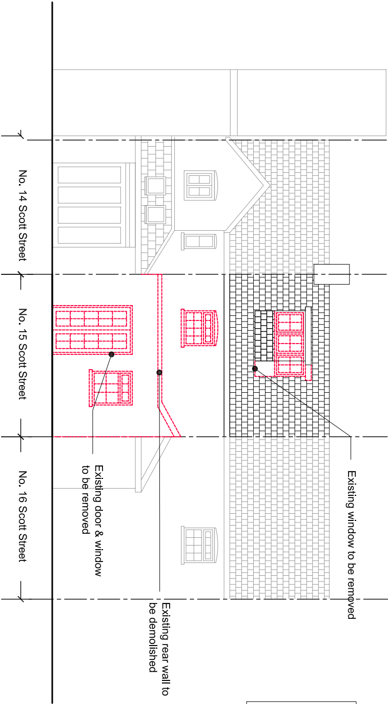
02 Existing South Elevation
