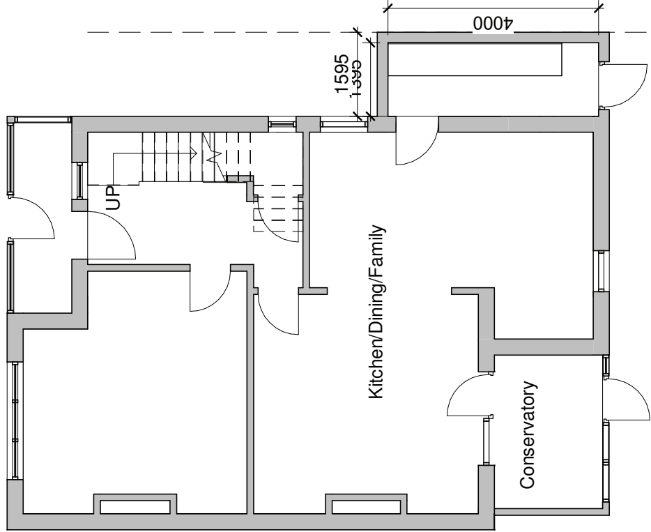
Proposed Ground Floor 1 : 100
