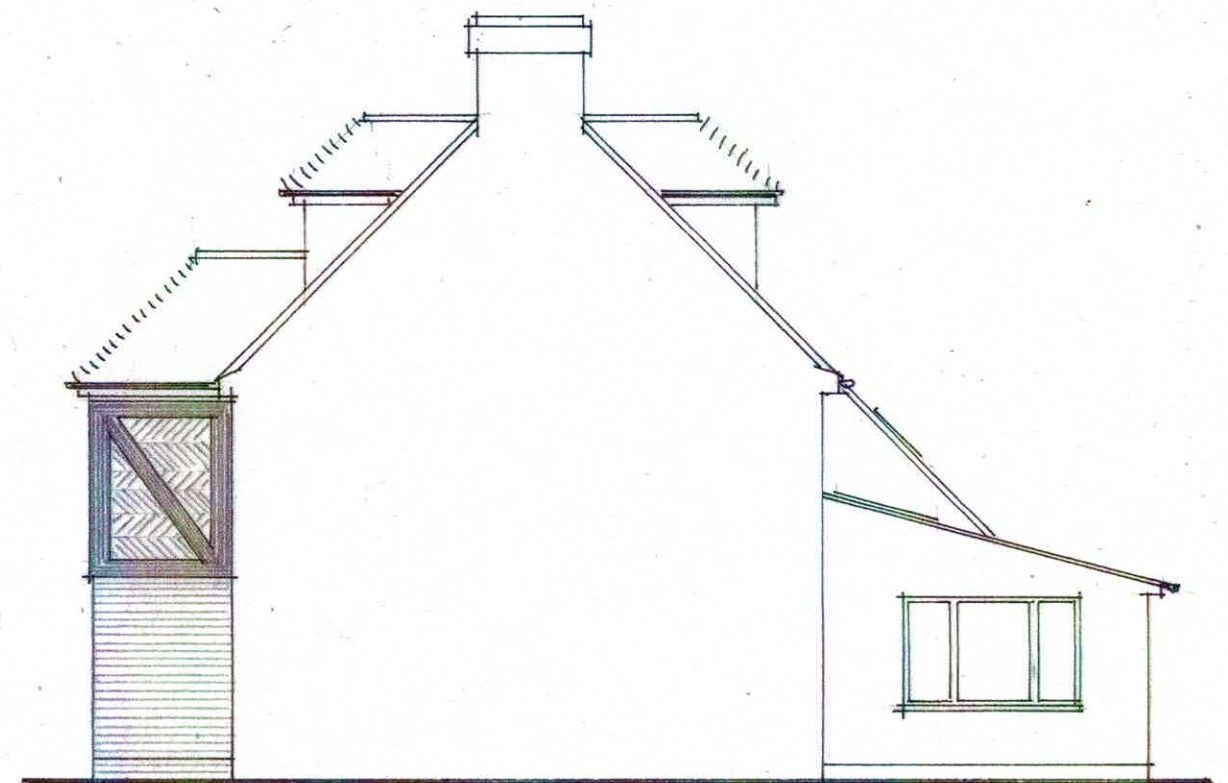
SIDE ELEVATION (NE) PROPOSED 1-100
