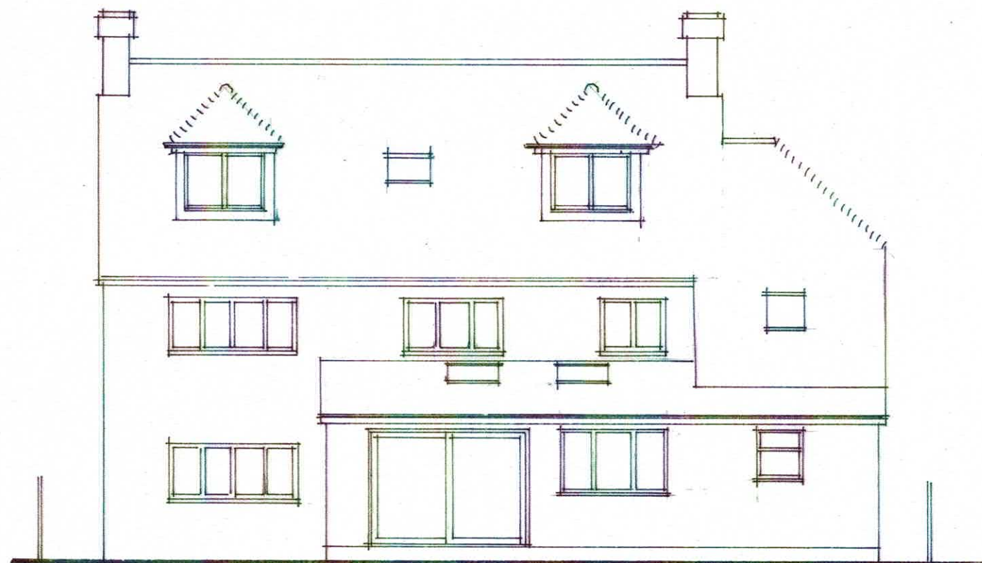
REAR ELEVATION (NW) PROPOSED 1-100
