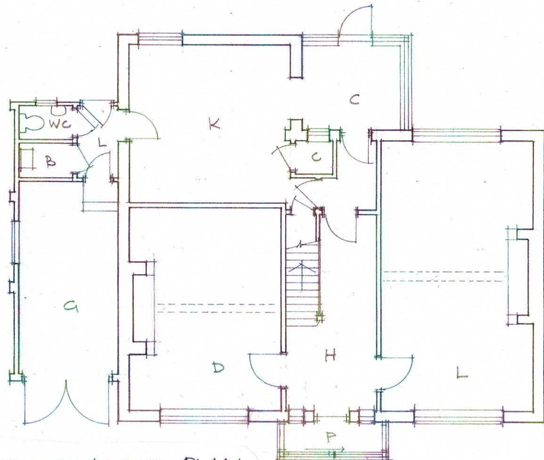
GROUND FLOOR PLAN EXISTING 1-100
