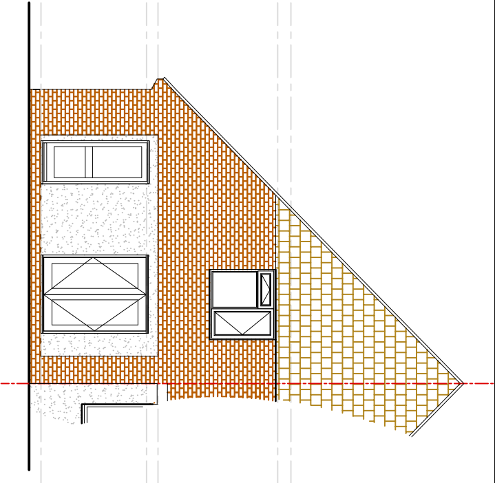
SOUTH ELEVATION - EXISTING.
