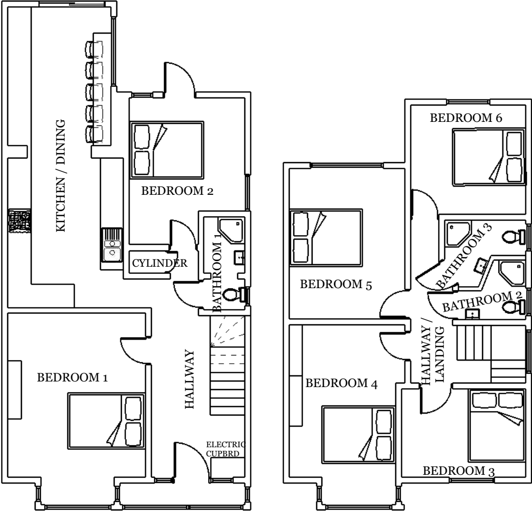
Proposed - 1st Floor
