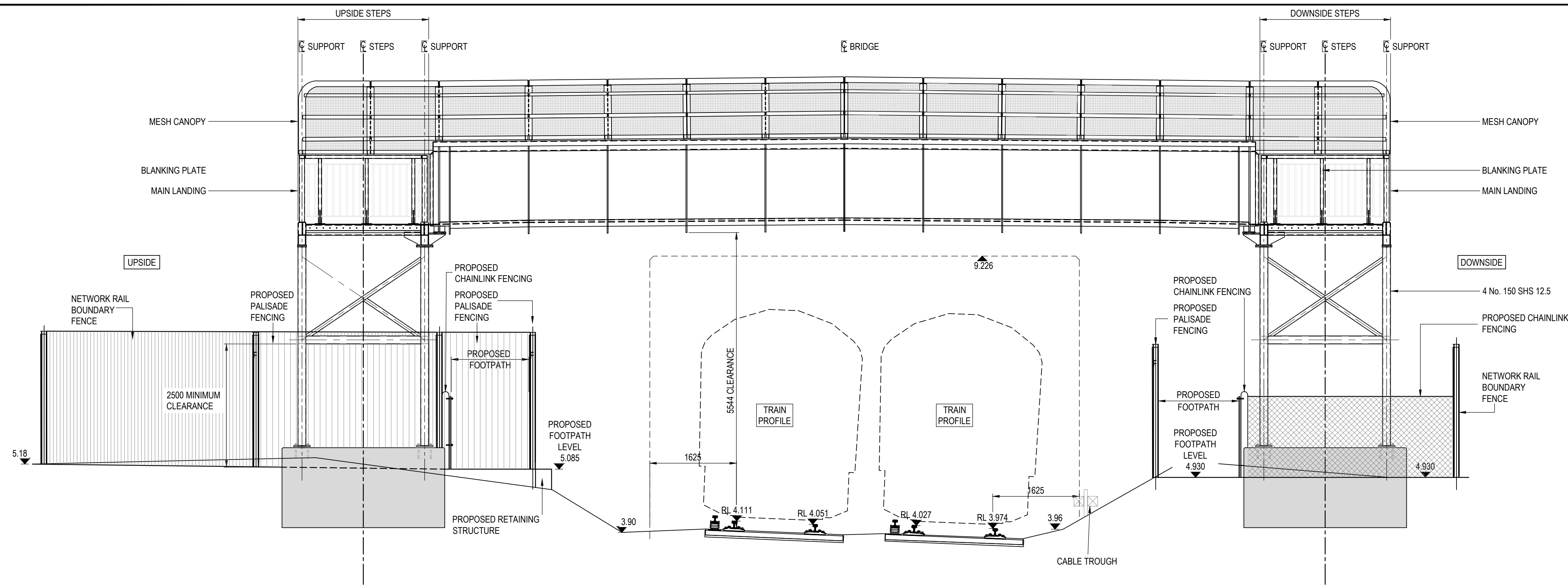
LONDON END ELEVATION SCALE 1:50
