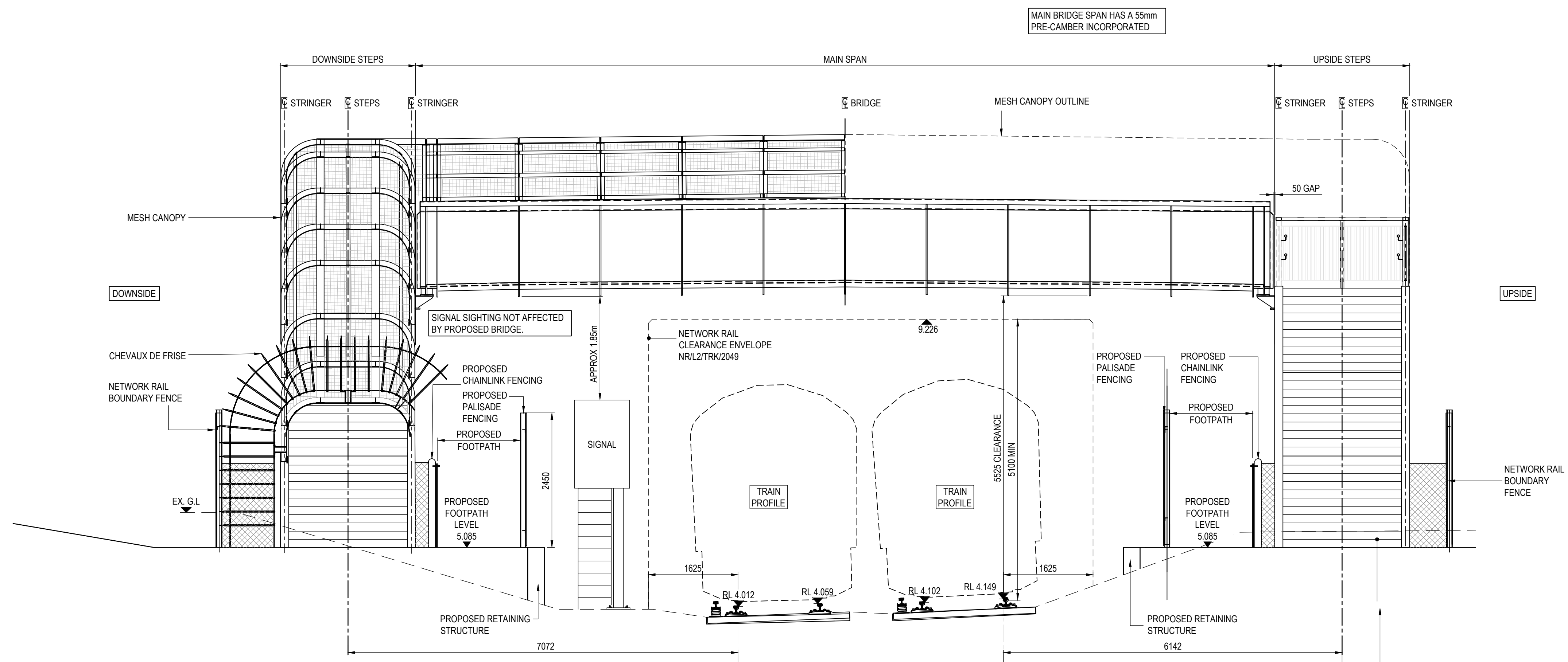
COUNTRY END ELEVATION SCALE 1:50
