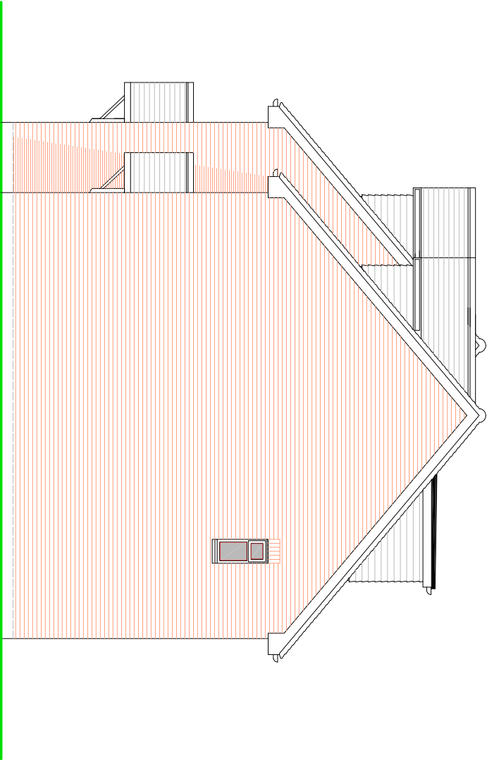
SIDE ELEVATION (WEST)
