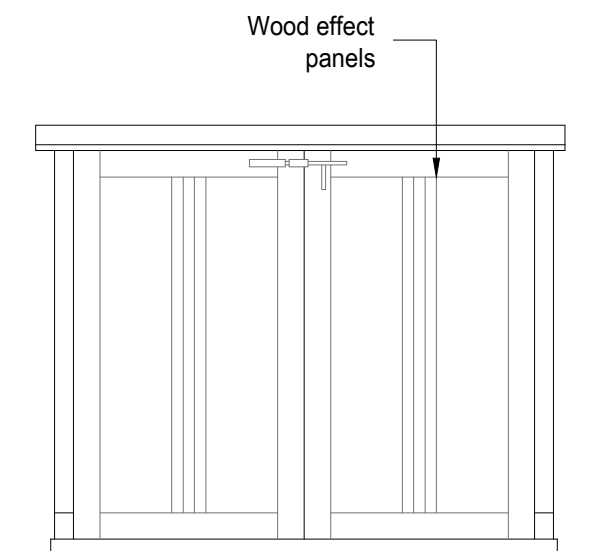
Proposed Bin Store Front Elevation 1:20
