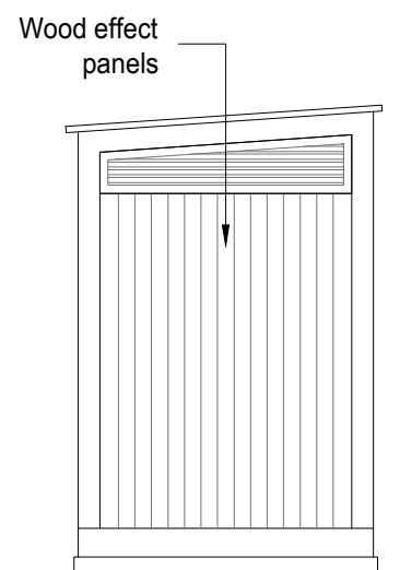
Proposed Bin Store Side Elevation 1:20
