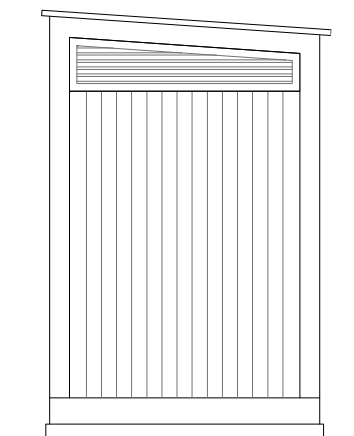
Proposed Bin Store Side Elevation 1:20
