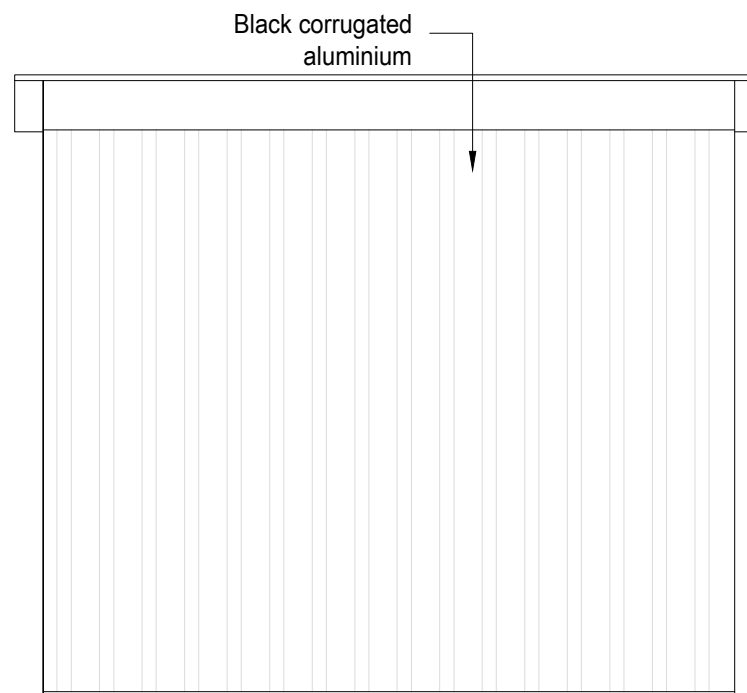
Proposed cycle rear elevation x4 1:20
