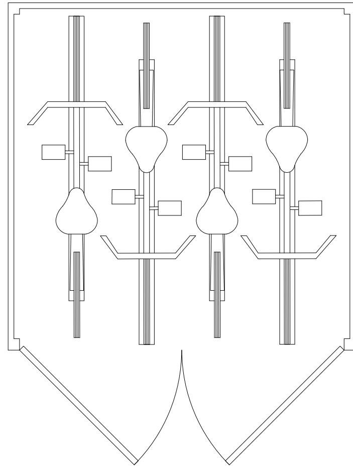
Proposed cycle store plan x4 (Duramax Bicycle Store) 1:20
