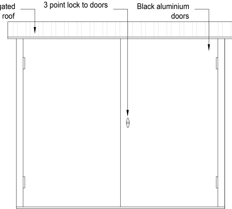
Proposed cycle front elevation x4 1:20
