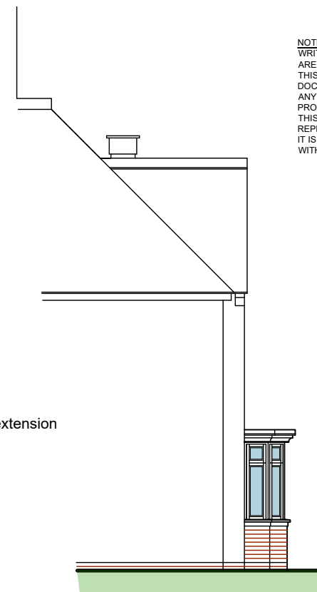
Part Side Elevation - East
