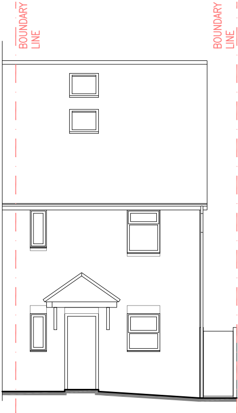
EXISTING NORTH-EAST FACING ELEVATION Sc. 1:100
