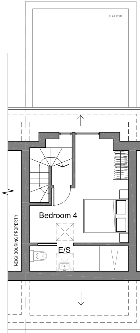
PROPOSED SECOND FLOOR PLAN Sc. 1:100
