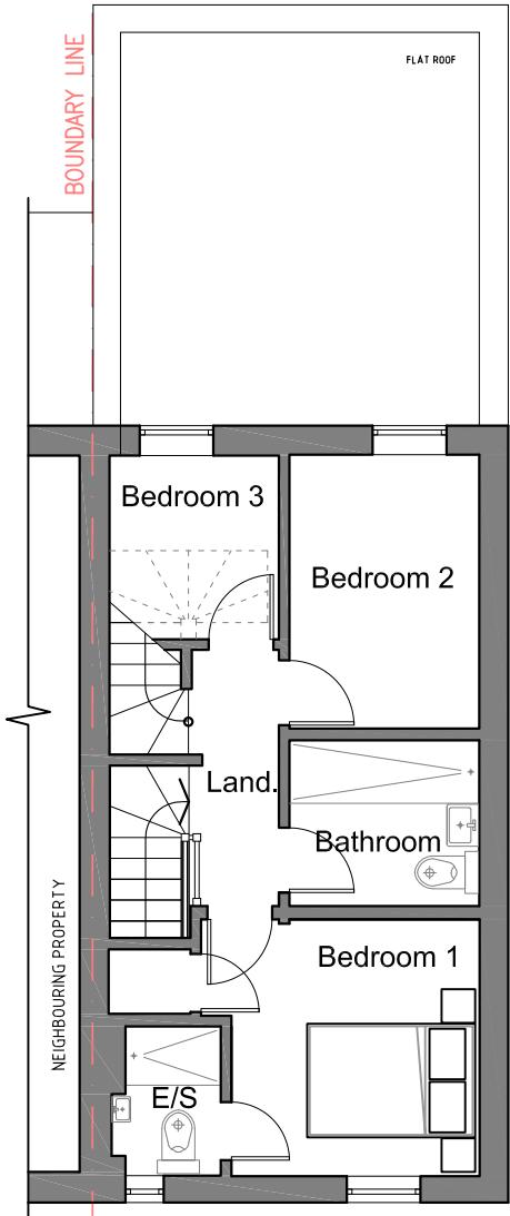
PROPOSED FIRST FLOOR PLAN Sc. 1:100
