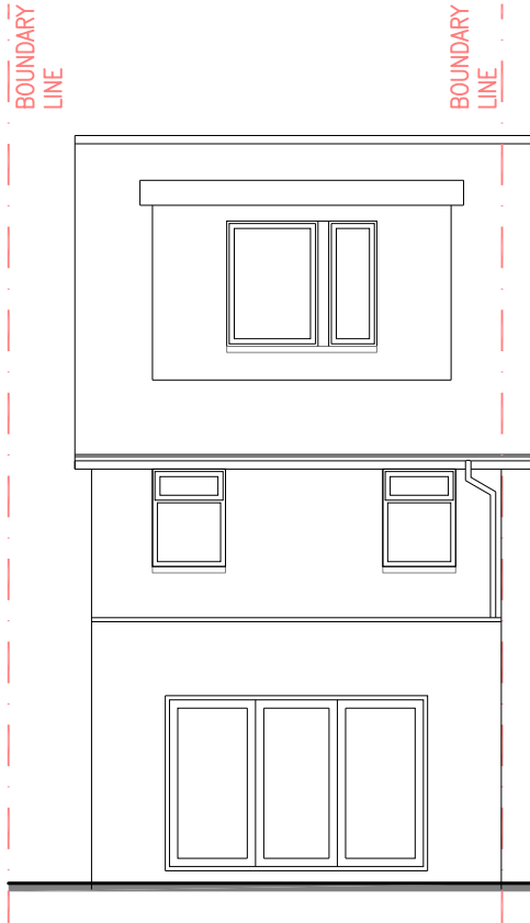
PROPOSED SOUTH-WEST FACING ELEVATION Sc. 1:100
