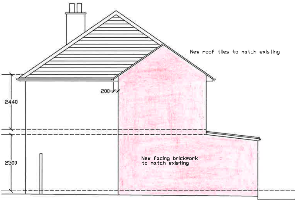
SIDE ELEVATION
