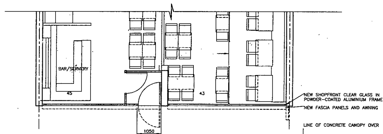
PROPOSED GROUND FLOOR LAYOUT.
