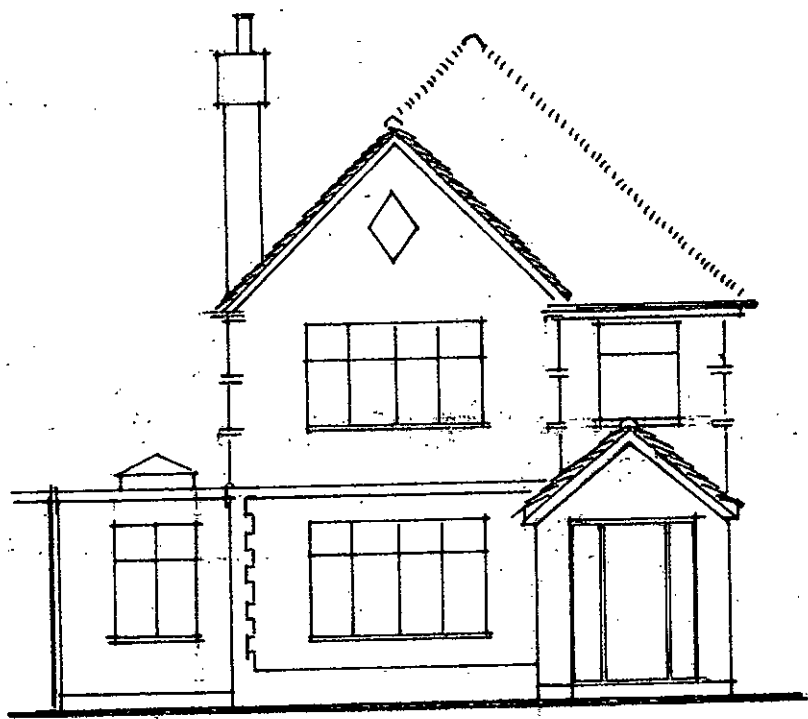
FRONT ELEVATION SOUTH 1:100
