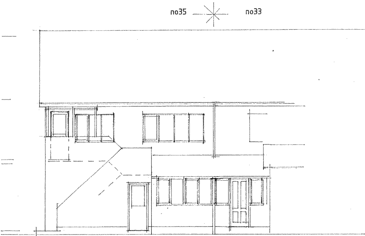
south elevation
