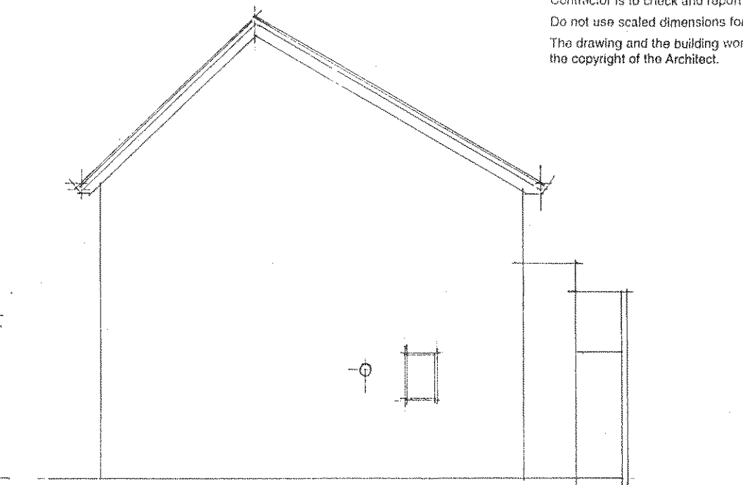
west elevation
