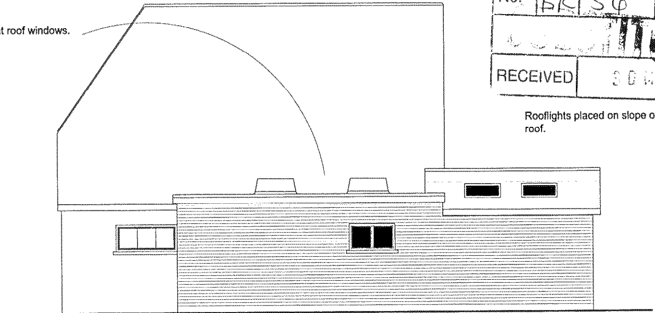
SIDE ELEVATION
