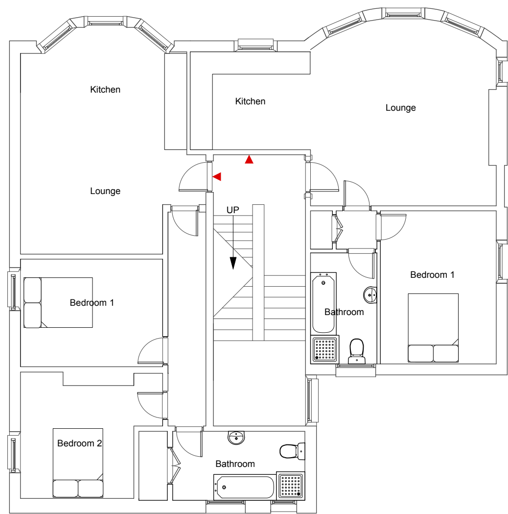
First Floor Plan (Proposed) 1:100
