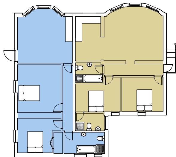
Basement Level 2 x 2 Bedroom Flats GIA's 66 sqm 72 sqm
