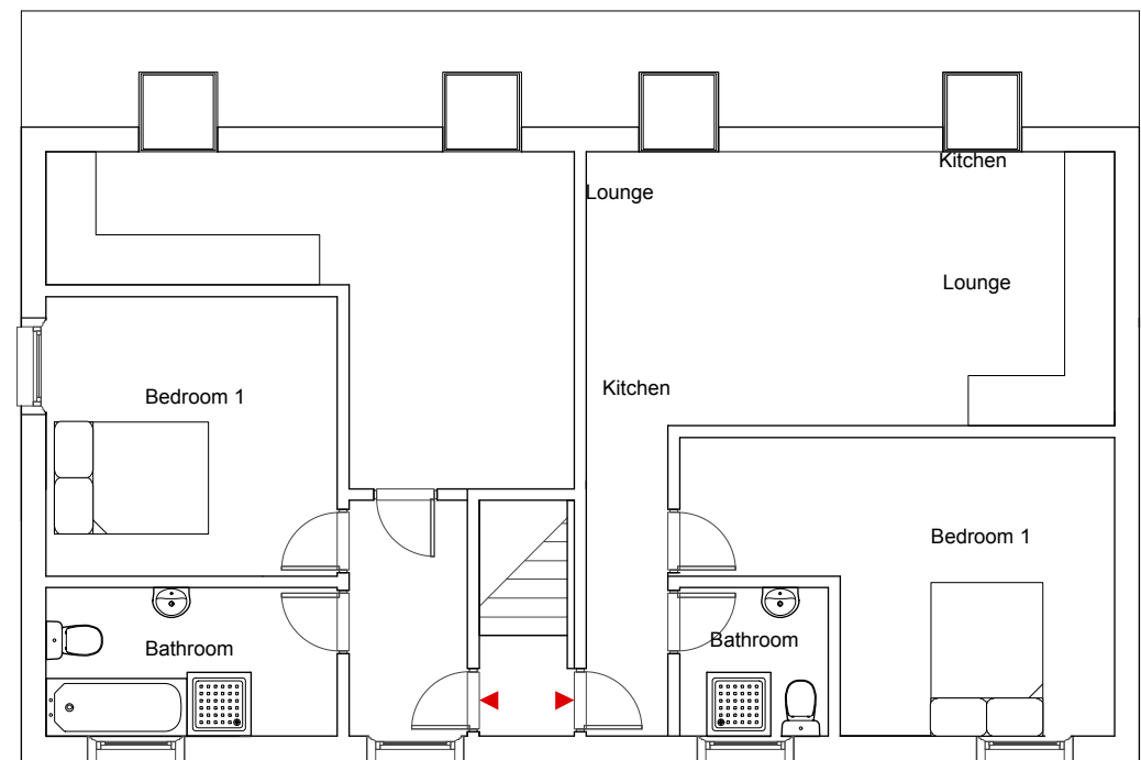
Second Floor Plan (Proposed) 1:100
