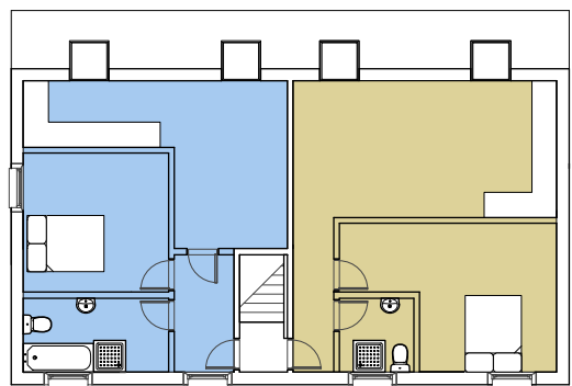
Second Floor Level 2 x 1 Bedroom Flats GIA's 40.8 sqm 44.6 sqm
