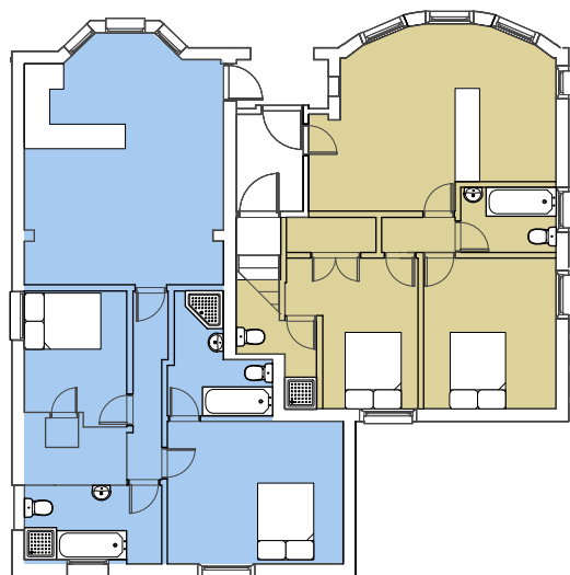
Ground Floor Level 2 x 2 Bedroom Flats GIA's 71 sqm 61 sqm
