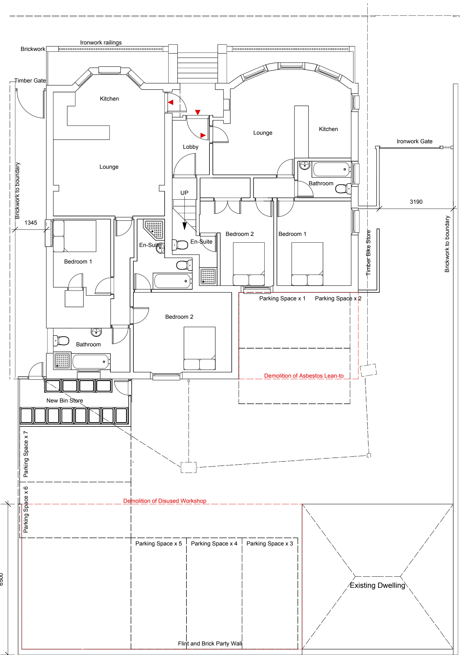
Site Plan (Ground Floor, Proposed) 1:100
