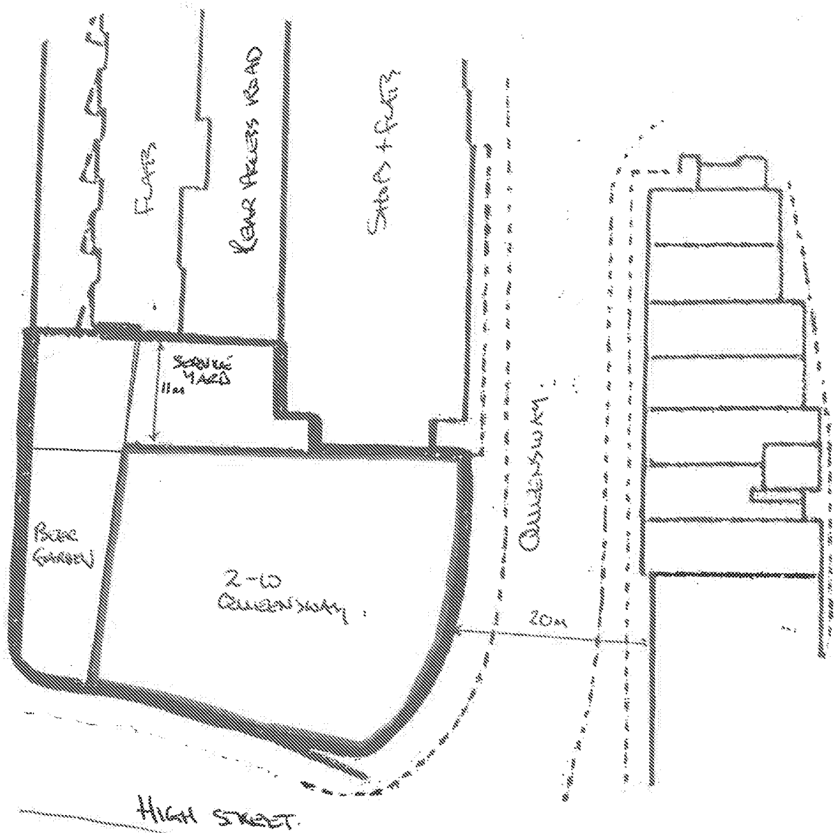
BLOCK PLAN (1:500) FIRST FLOOR
