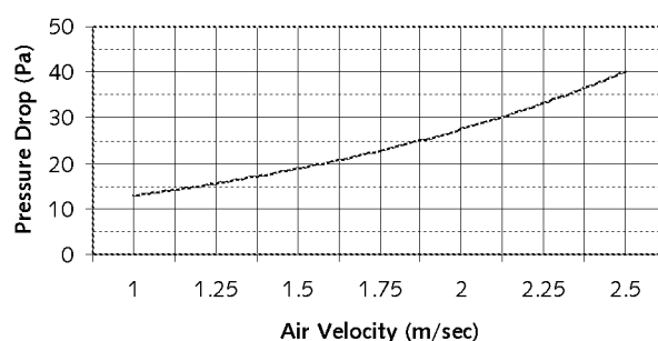
Pressure Drop vs/ Face Velocity Type 90 TA1 Panel Filter 20mm Thick
