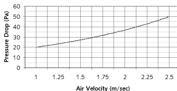
Pressure Drop vs/ Face Velocity Type 90 TA2 Panel Filter 45mm Thick
