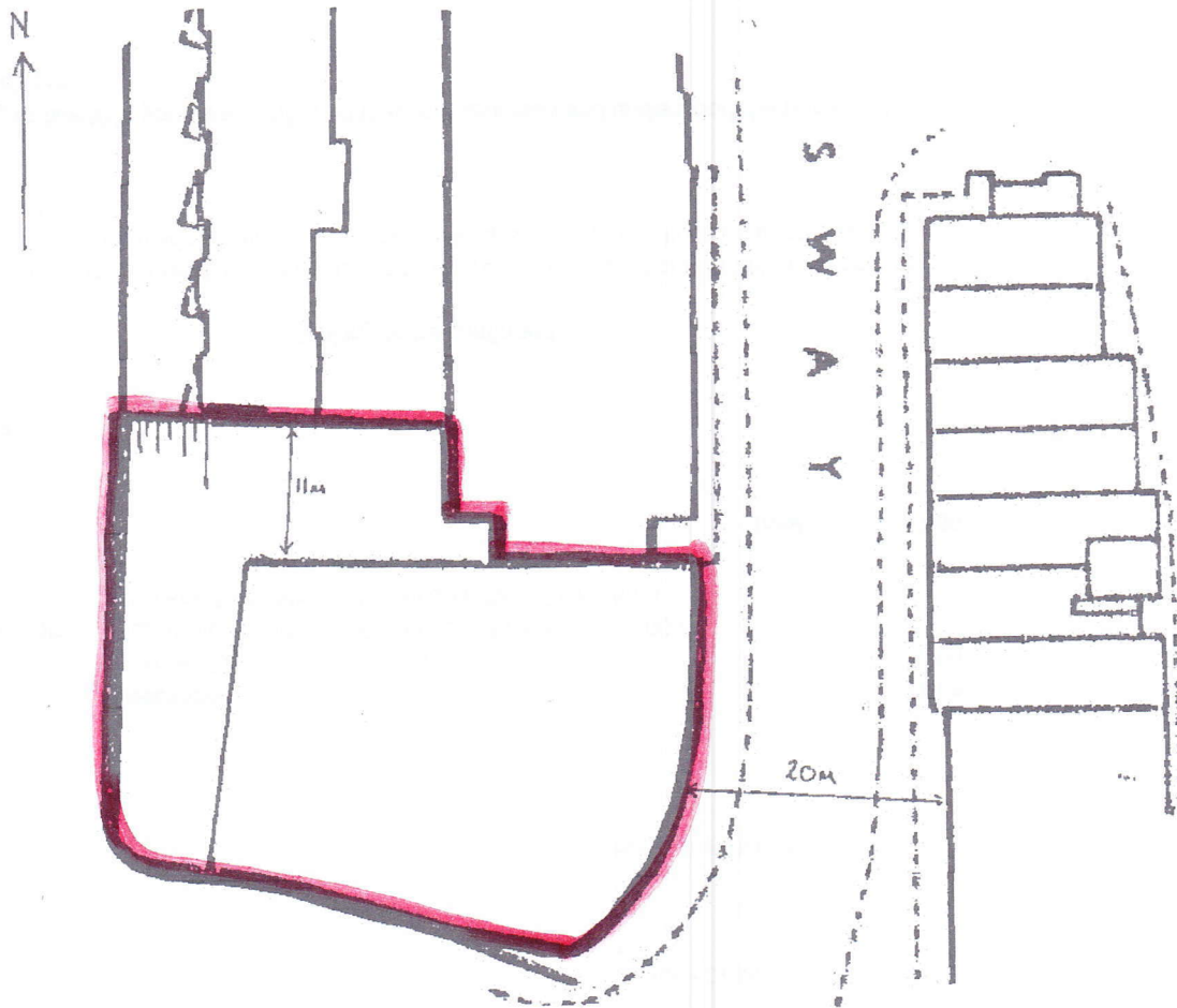
BLOCK PLAN (1:500)
