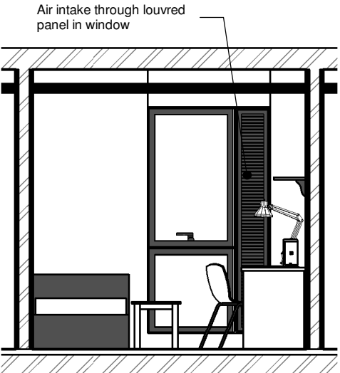
Typical Bedroom Section 3 1 : 50
