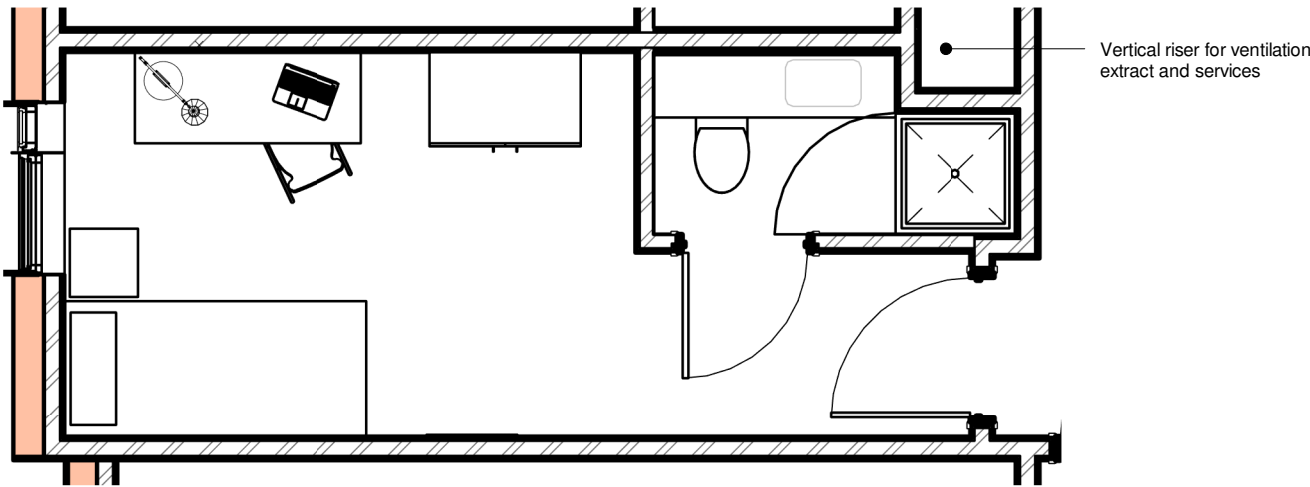
Typical Bedroom Layout 1 : 50
