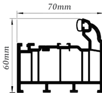
Outer Frame
