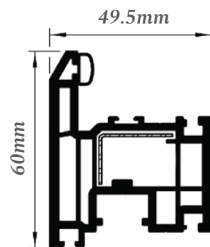
Flush Casement
