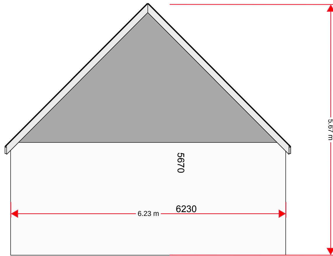
Side Elevation
