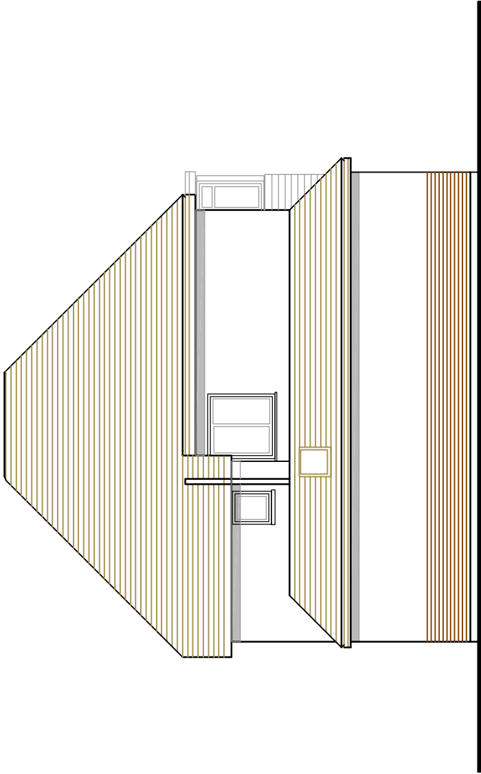
PROPOSED WEST ELEVATION 1:100
