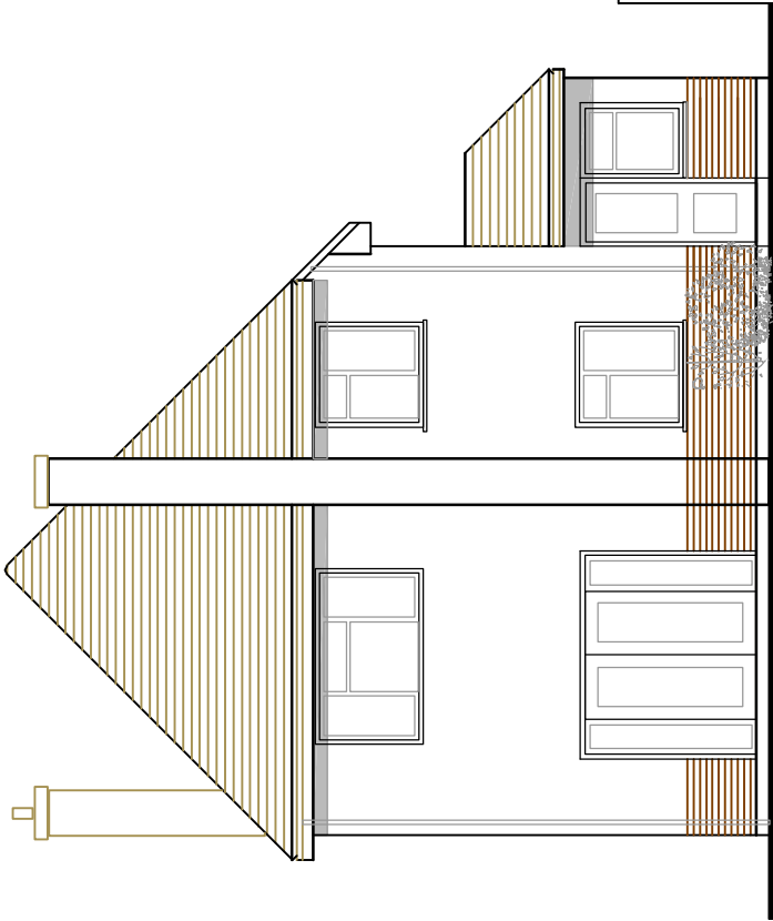
PROPOSED NORTH ELEVATION 1:100
