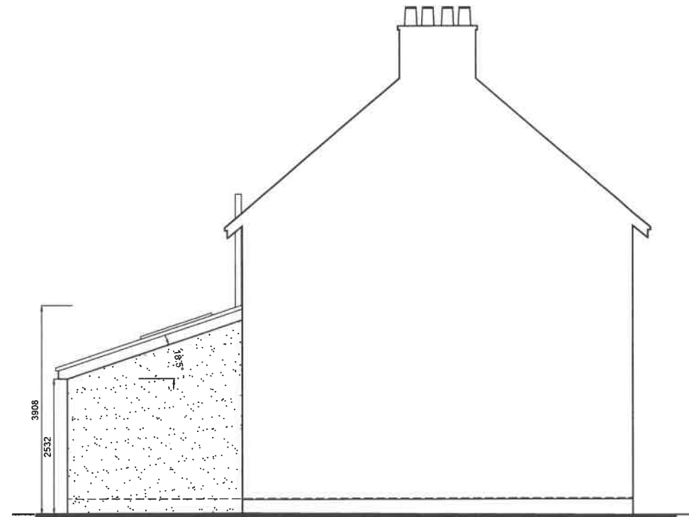
LEFT (NORTH-EAST)
