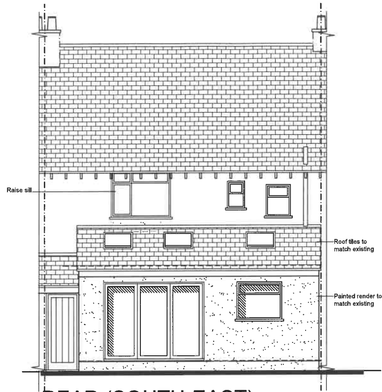
REAR (SOUTH-EAST)
