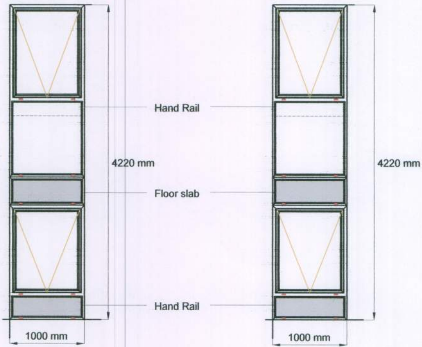
Proposed North Staircase - North Elevation Proposed North Staircase - South Elevation
