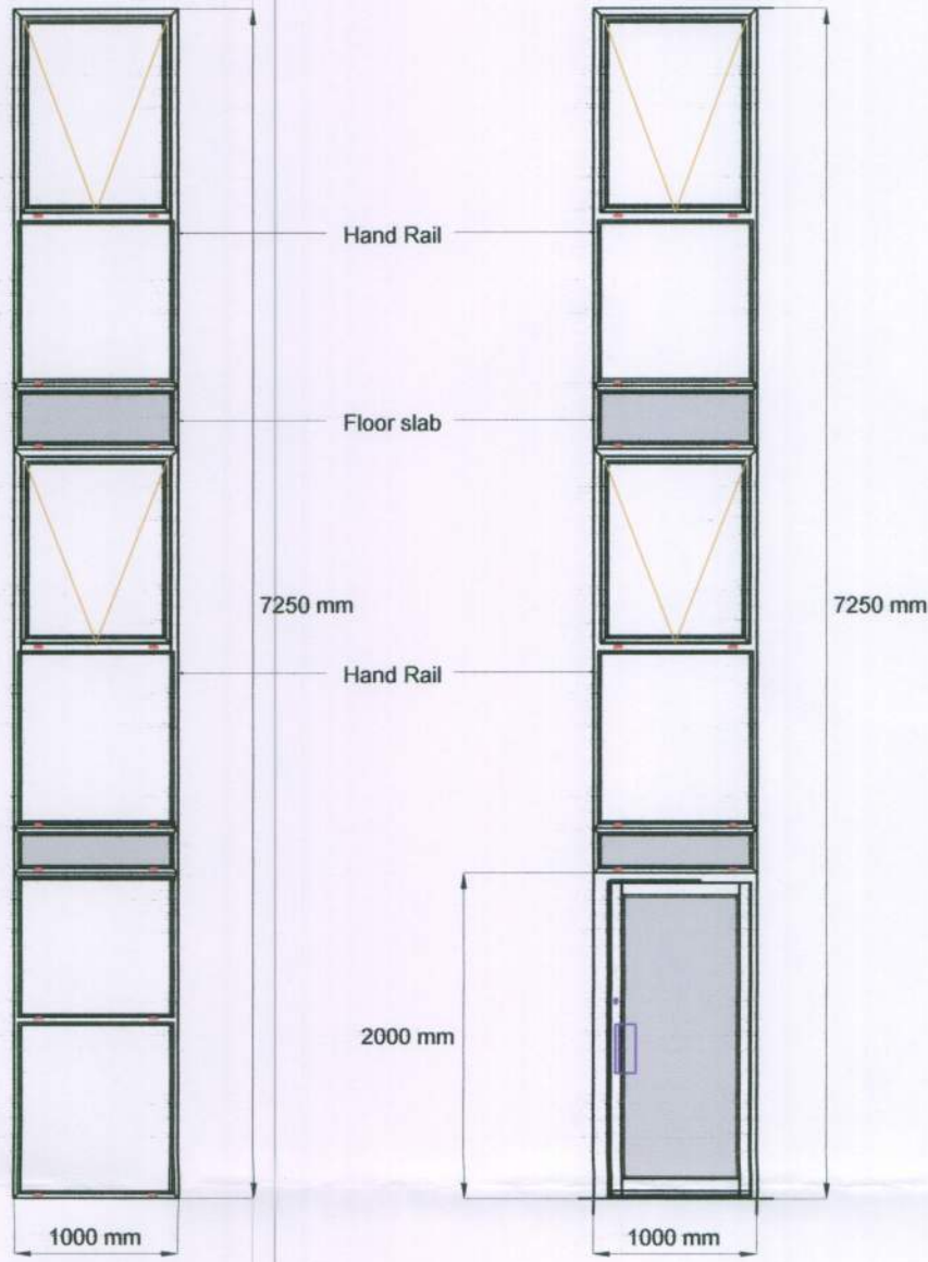
Proposed South Staircase - North Elevation Proposed South Staircase - South Elevation
