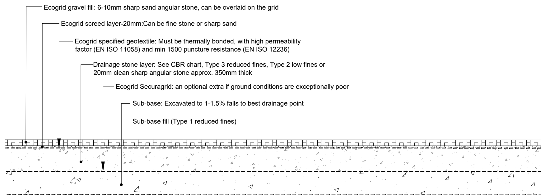
Typical Section Through General Car Park Circulation Areas
