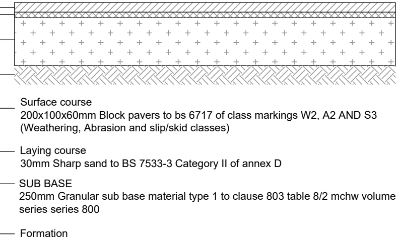
Block paved driveway construction To be read in accordance with NHBC standards chapter 10.2
