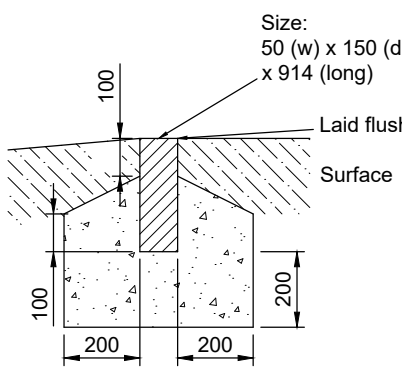
Edging Type EF flat top (1:10)
