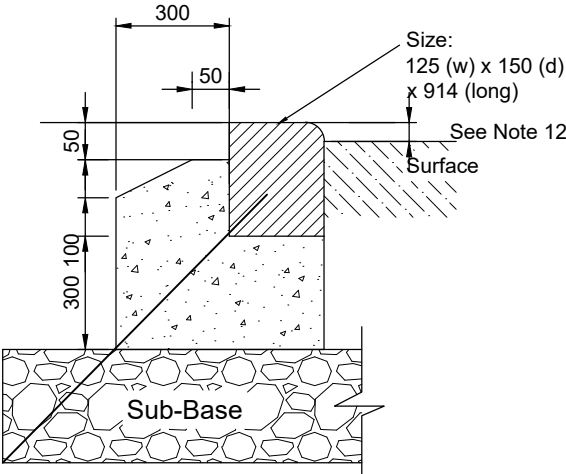
Drop kerb Type BN (1:10)
