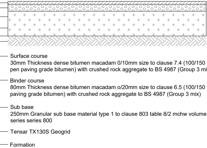
Flexible private carriageway construction To be read in accordance with NHBC standards chapter 10.2
