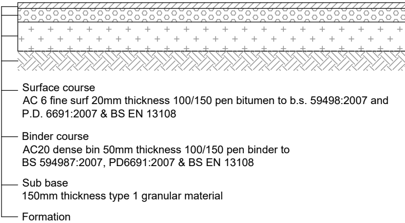
Flexible footway construction
