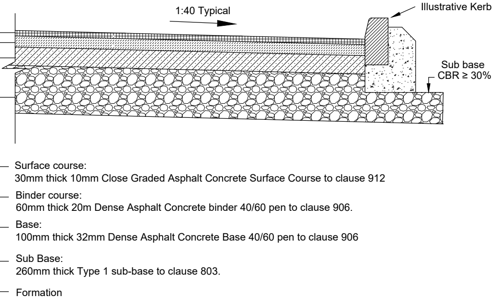
Flexible adopted carriageway construction
