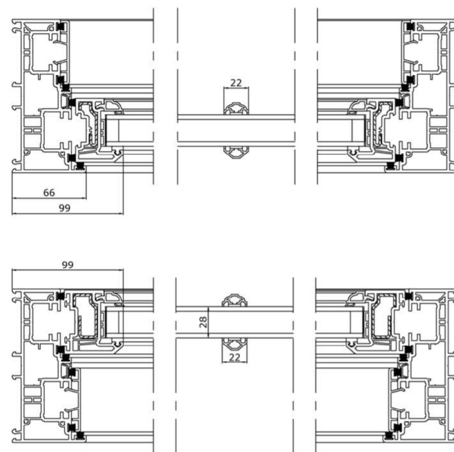
TYPICAL WINDOW DETAIL
