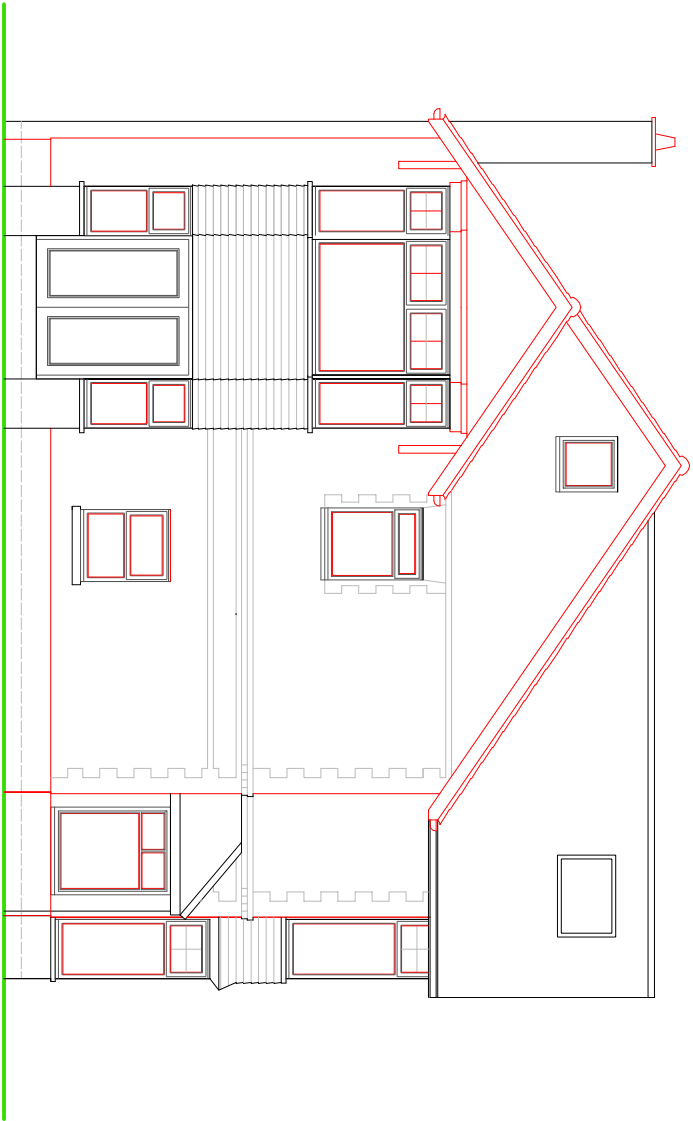
SIDE ELEVATION
