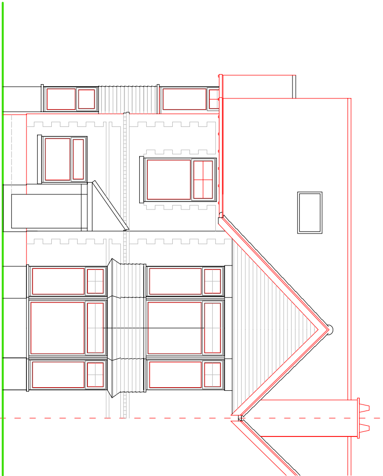
FRONT ELEVATION
