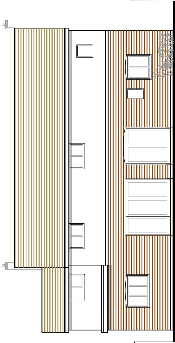
PROPOSED NORTH ELEVATION 1:100
