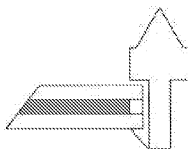
Full size section standard glazing bar with Slimlite
