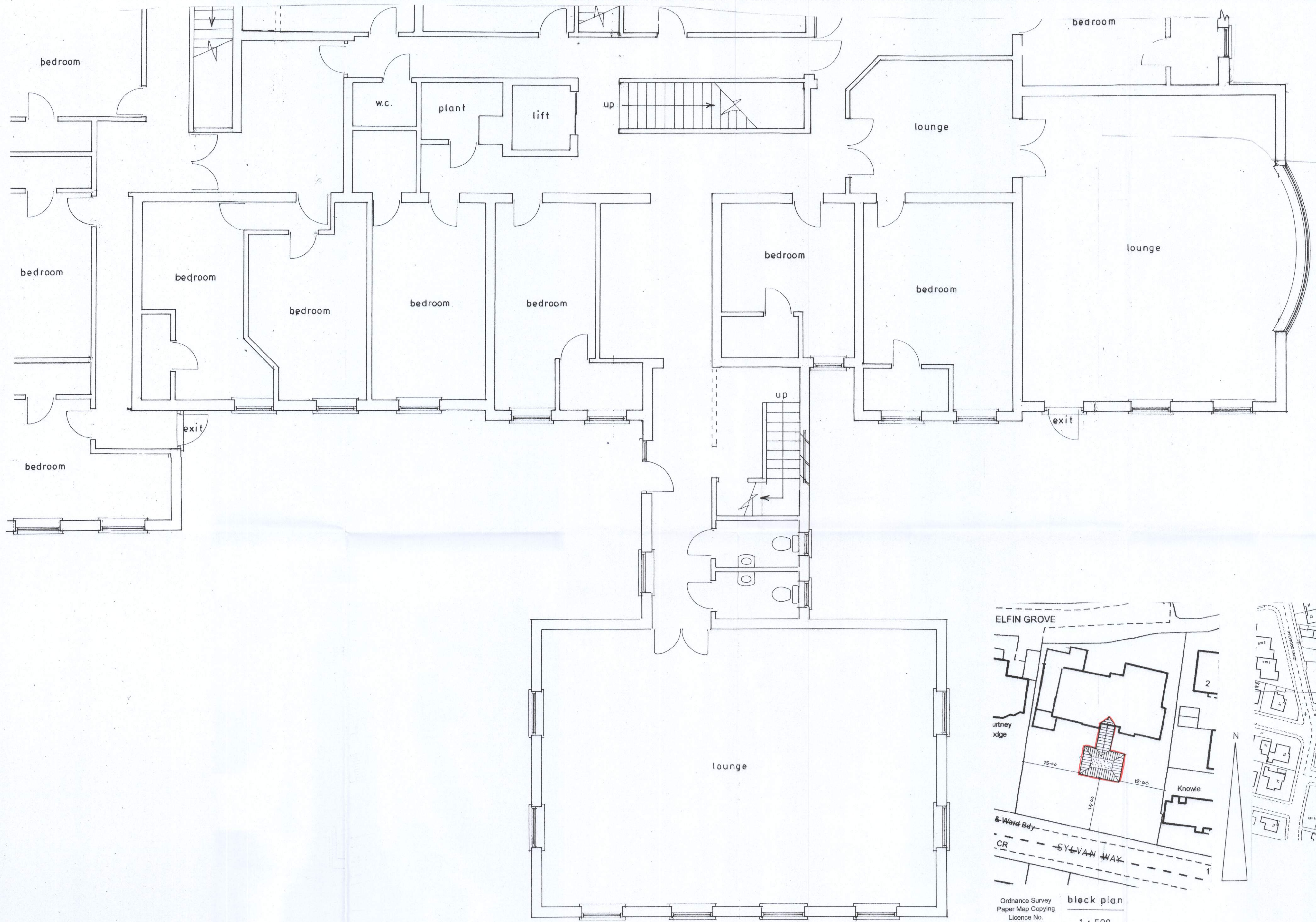
Ground floor plan 1 : 50
