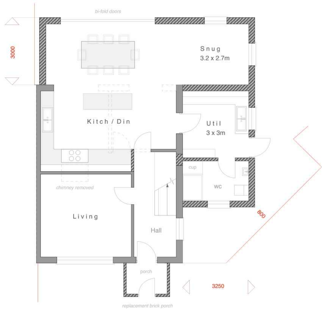
Proposed GF Plan at 1:100 scale
