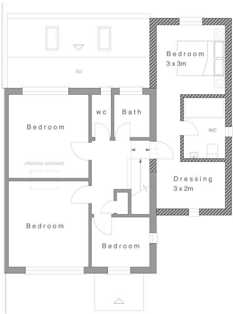
Proposed FF Plan at 1:100 scale
