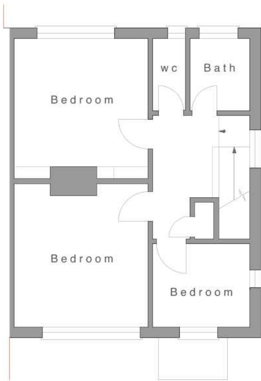
Existing FF Plan at 1:100 scale
